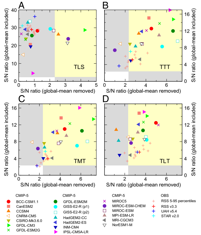
Fig. 9. Summary plot of S/N ratios for (A) TLS, (B) TTT, (C) TMT, and (D) TLT. Results are for trends over the entire 33-y satellite record (1979–2011). The D&A analysis was performed in two different ways: with removal of the global mean component of temperature change from each model and observational dataset, and with the global mean change included. Results for these two processing choices are plotted on the x and y axes, respectively. The S/N analysis relies on the O3+V fingerprints (estimated using multimodel average temperature changes from 1861 to 2011) and the TOP-5 model noise estimates. The yellow shading denotes the region where S/N ratios are significant at the 1% level or better for both the global mean removed and global mean included cases. In the gray shaded regions, statistically significant S/N ratios are obtained in only one of these two cases. See Figs. 7 and 8 and SI Appendix for additional information.
