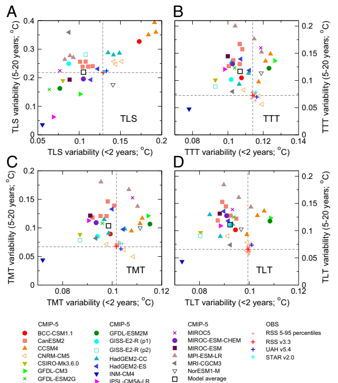
Fig. 5. Comparison of simulated and observed variability of monthly mean near-global anomalies in (A) TLS, (B) TTT, (C) TMT, and (D) TLT. In each panel, the monthly to interannual timescale variability of detrended, high pass-filtered temperature data ( s_{\text{HIGH}} , x axis) is plotted against the 5- to 20-year timescale variability of band pass-filtered data ( s_{\text{LOW}} , y axis). The dashed lines are centered on the observed values of s_{\text{HIGH}} and s_{\text{LOW}} for version 3.3 of the RSS dataset. The multimodel average s_{\text{HIGH}} and s_{\text{LOW}} values were calculated by averaging over the ensemble mean s_{\text{HIGH}} and s_{\text{LOW}} results for each of the 20 individual CMIP-5 models. The same 396 months (January 1979 to December 2011) were used for the analysis of observations and synthetic MSU temperatures from the spliced historical/RCP8.5 runs.
