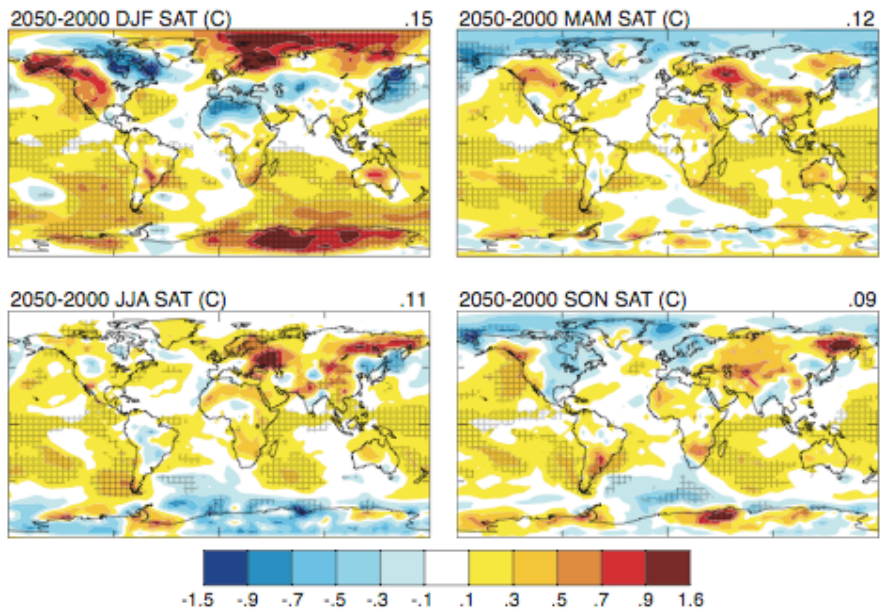
3 4 Figure 9. Ensemble mean seasonal average surface air temperature ( ^{\circ}\text{C} ) changes induced 5 by the short-lived species near 2050 based on the last 11 years of the transient ensemble 6 simulations. Numbers in the upper right corners give the global mean. Hatching indicates 7 95% significance. 8
