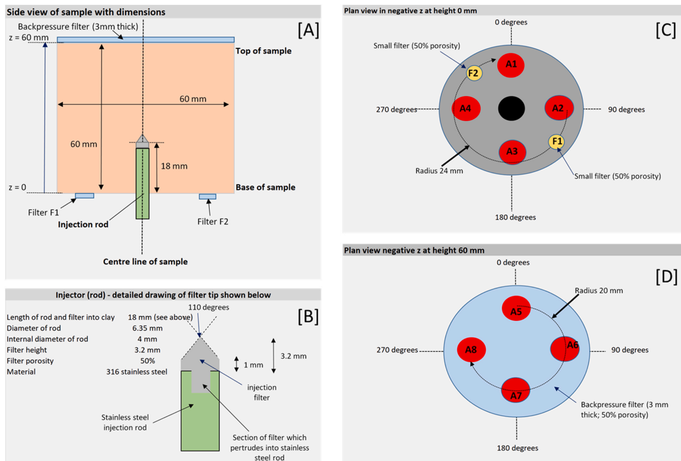
Fig. 2. Schematic of apparatus. [A] shows the dimensions of the sample and filters. [B] shows the dimensions of the injection filter. [C] and [D] show the location of the axial sensors in contact with the base and top of sample respectively.
