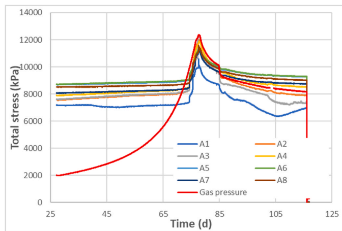
Fig. 6. Test FPR-21–004 showing the development of gas pressure and axial stress, stage 5. The gradual increase in most sensors from day 28 to 70 can be attributed to continued hydration of the bentonite.
