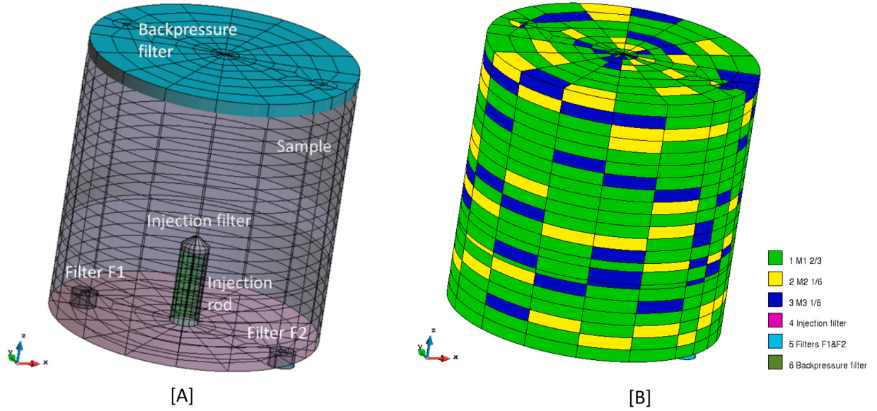
Fig. 16. 3D mesh (with 3430 elements and 3909 nodes) used by CIMNE-UPC/Andra to simulate the test: [A] shows the modelled sample mesh and the main component details and [B] shows the material heterogeneity (2/3–1/6–1/6 weighting).
