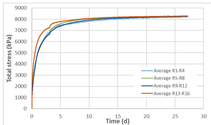
Fig. 5. Test FPR-21–004 showing the development of radial stress at each plane of measurement during test stages 1 and 2. The position of each ‘array’ is in Table 1.
