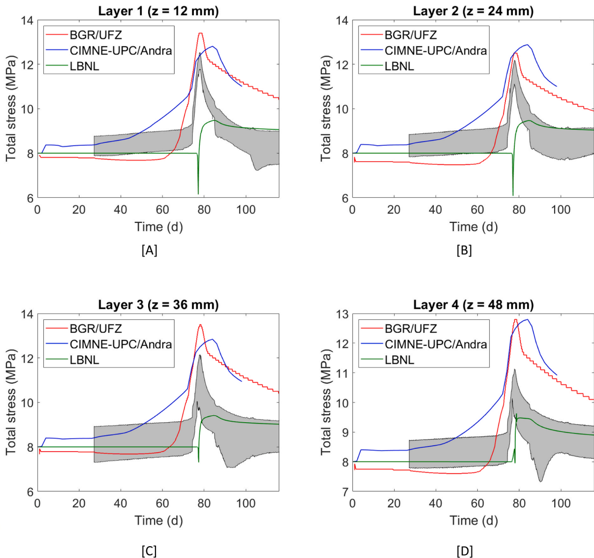
Fig. 18. Radial stresses obtained at each layer with the three numerical models. Grey zones represent experimental radial stresses.
