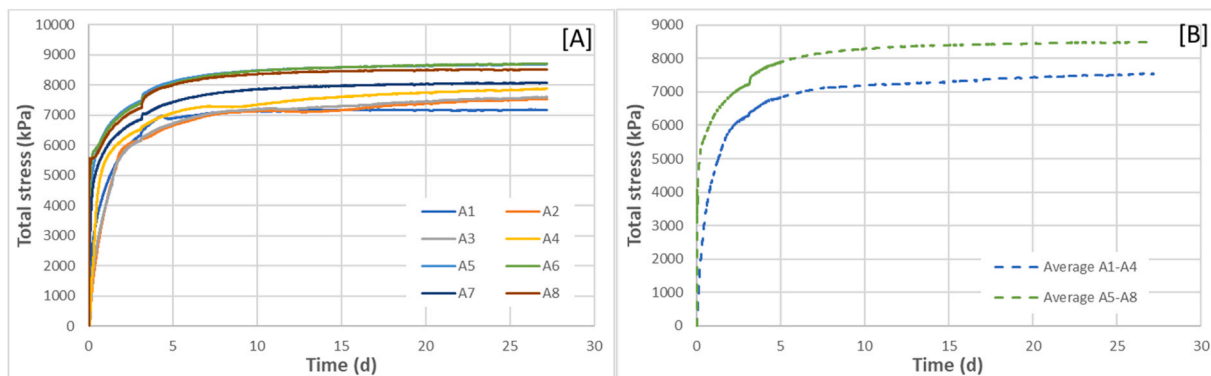
Fig. 3. Test FPR-21-004 showing the development of axial stress during test stages 1 and 2. In [A] each sensor is shown and in [B] the average stress is shown: sensors A1 to A4 (located at the base of the sample) and A5 to A8 (positioned on the top face of the sample).
