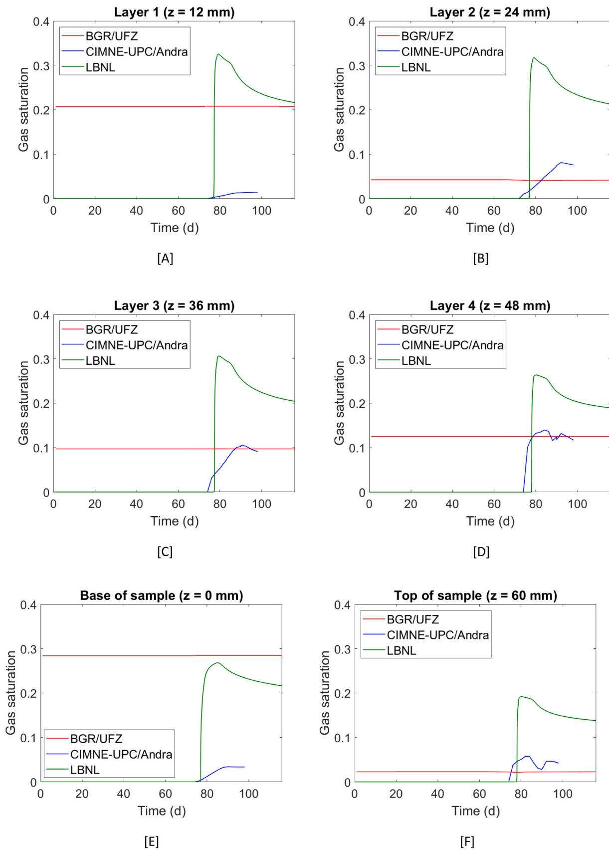
Fig. 22. Average gas saturation profiles at each layer, at the base and at the top of the sample obtained with the three numerical models.
