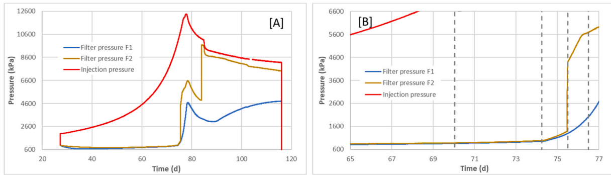
Fig. 13. [A] pore pressure development in filters F1 and F2 during test FPR-21-004. [B] expanded data from day 65 to day 77 showing the filter response during initial gas entry, major gas entry, initial gas breakthrough and major gas breakthrough respectively from left to right.
