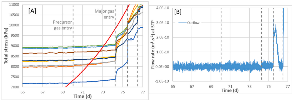
Fig. 7. Data from part of stage 4 of test FPR-21-004 with dotted lines denoting significant events. [A] expanded view of gas pressure and axial stress data showing precursor gas entry around day 70.1 followed by major gas entry at day 74.3. Line colours are the same as those on Fig. 6. [B] shows time averaged outflow data under experimental conditions with major gas outflow occurring at day 75.5.
