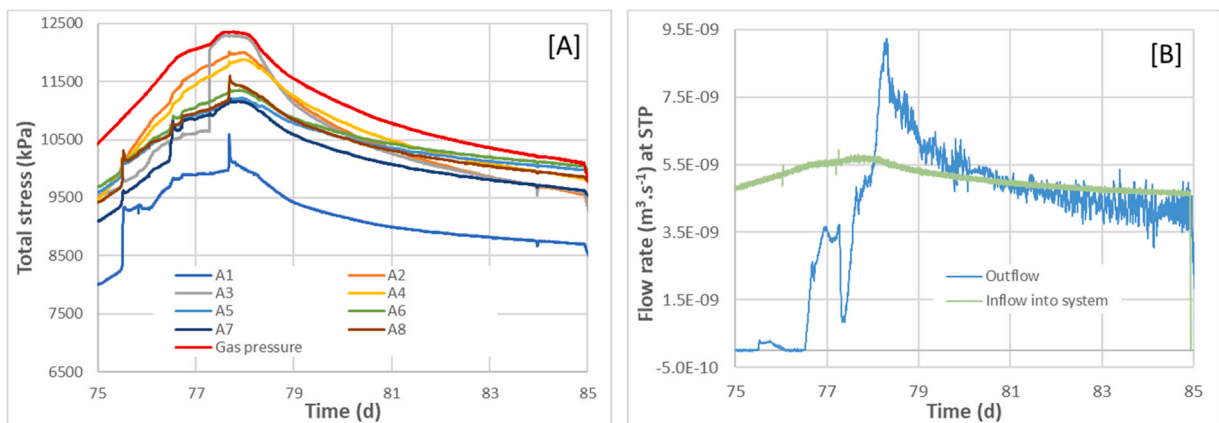
Fig. 8. Data from part of stage 4 of test FPR-21-004. [A] development of axial stress and [B] evolution of inflow and outflow data at STP, from day 75–85. Combined, the data illustrates the complex coupling between development of flow and accompanying changes in stress within the bentonite.
