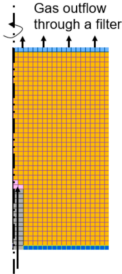
Fig. 15. Axisymmetric mesh (with roughly 900 elements, including element representing the injection filter and the injection chamber) used by LBNL.
