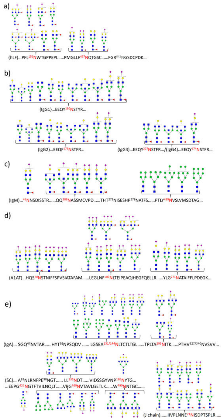
Fig. 2. Glycan site-heterogeneity of human milk glycoproteins: a LF, b IgG, c IgM, d A1AT, and e sIgA. Green circles, yellow circles, blue squares, red triangles, and purple diamonds represent mannose, galactose, GlcNAc, fucose, and NeuAc residues, respectively
