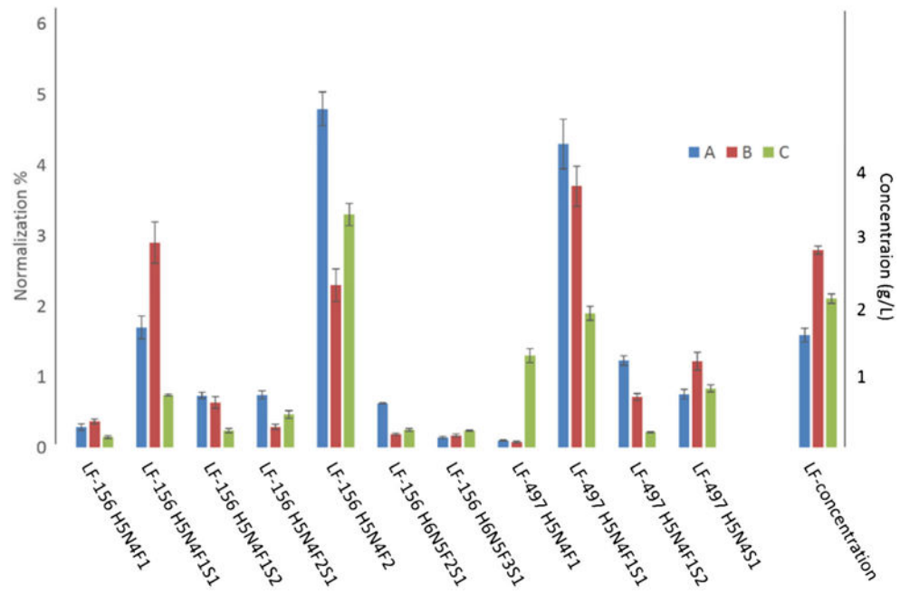
Fig. 5. Eleven normalized LF glycopeptide abundances monitored from three milk samples ( a , b , and c ). LF concentration (g/L) of three milk samples on the right of the plot. Normalization was performed with the ratio between glycopeptide signal peak area and the LF peptide peak area. This suggests the dynamic variation on site-specific glycosylation. Error bars are representative of reproducibility from replicates on different days
