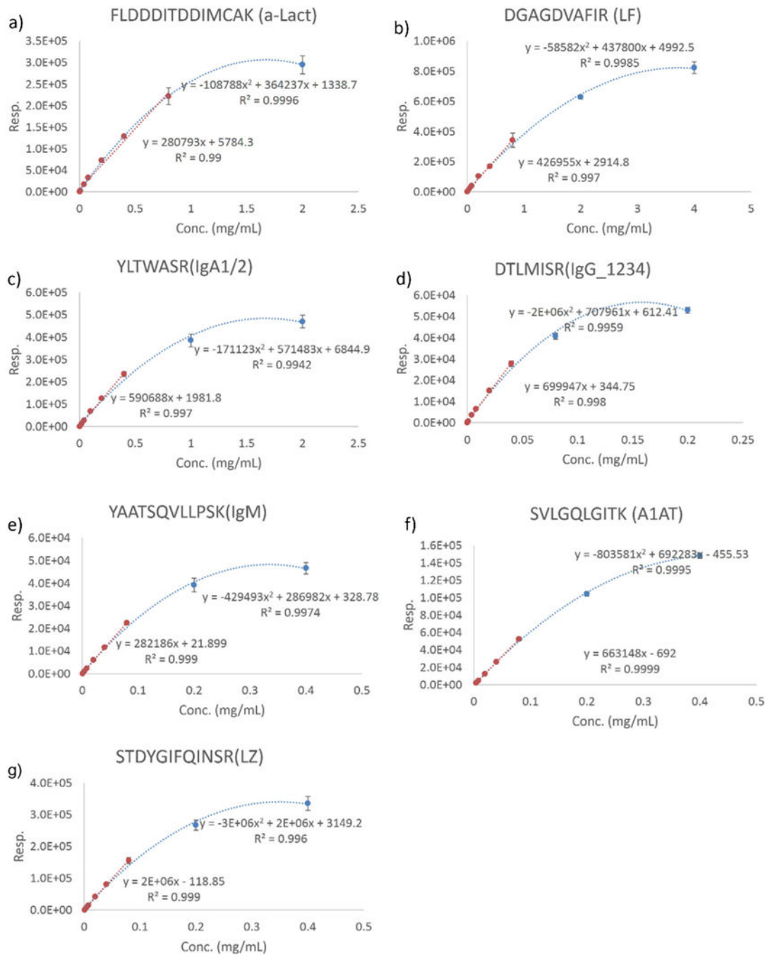
Fig. 4. Peptide calibration curves for protein quantitation. a α-lact, b LF, c IgA1/2, d IgG1234, e IgM, f A1AT, and g LZ. The response can be fitted to a quadratic equation ( dashed in blue ). The dynamic range was over 1000. The linear fit ( dashed in red ) generated an equation with R^2 from 0.99 to 0.999. The linear range was more than 100
