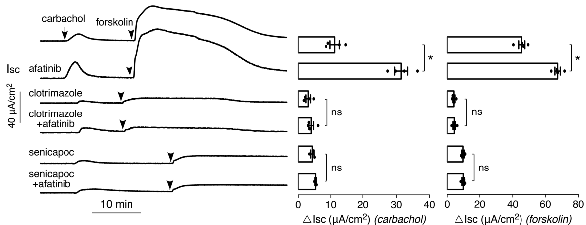
Figure 6. K + channel inhibitors block the afatinib-induced augmentation in carbachol current. (Left) short-circuit current in T84 cells treated with 20 μM afatinib, 30 μM clotrimazole, and/or 10 μM senicapoc, as indicated, 30 minutes before addition of 100 μM carbachol followed by 10 μM forskolin. (Right) summary of peak carbachol- and forskolin-induced peak current (mean ± SEM, n = 3-4 ; * P < 0.05 , by 2-tailed t test).
