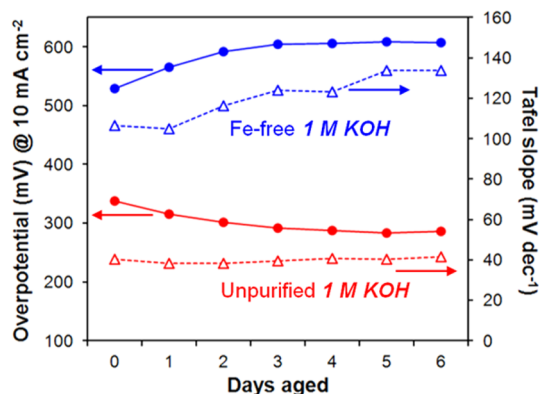
Figure 4. Effect of aging on the overpotential at 10 \text{ mA cm}^{-2} geometric current density (filled circles) and Tafel slope (open triangles) for \text{Ni}(\text{OH})_2 films deposited on polished Au-RDEs aged in Fe-free (blue) vs unpurified (red) 1 \text{ M KOH} .
