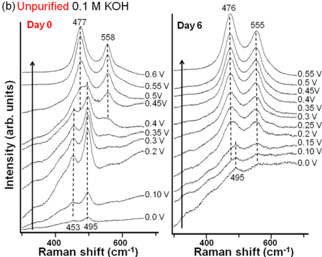
Figure 6. In situ Raman spectra collected over Ni(OH) 2 /NiOOH films deposited on roughened Au in (a) Fe-free and (b) unpurified 0.1 M KOH on Day 0 and Day 6. Potentials are reported vs Hg/HgO. The oxygen evolution equilibrium potential is 0.365 V vs Hg/HgO in 0.1 M KOH.
