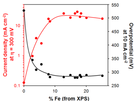
Figure 5. Oxygen evolution activity of electrodeposited NiOOH films deposited on Au RDEs at 300 mV overpotential and 10 \text{ mA cm}^{-2} geometric current density in 1 M KOH as a function of Fe content. Curves are included to guide the eye.
