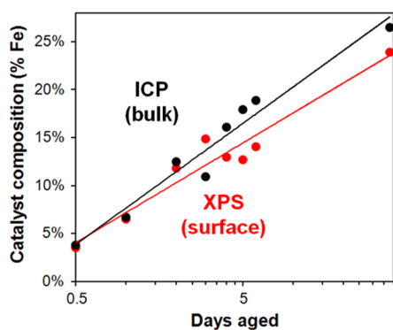
Figure 3. Iron content of \text{Ni}(\text{OH})_2 films deposited on polished Au-RDEs measured from X-ray photoelectron spectroscopy (XPS) and inductively coupled plasma optical emission spectroscopy (ICP-OES) vs days aged in unpurified 1 \text{ M KOH} . Lines show a logarithmic best-fit ( y = a \ln(x) + b ) to each data set. Values of a and b for each data set can be found in the Supporting Information file.
