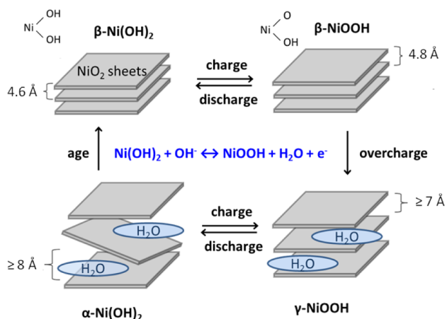
Figure 1. Bode scheme 28 for the Ni(OH) 2 /NiOOH redox transformation.
