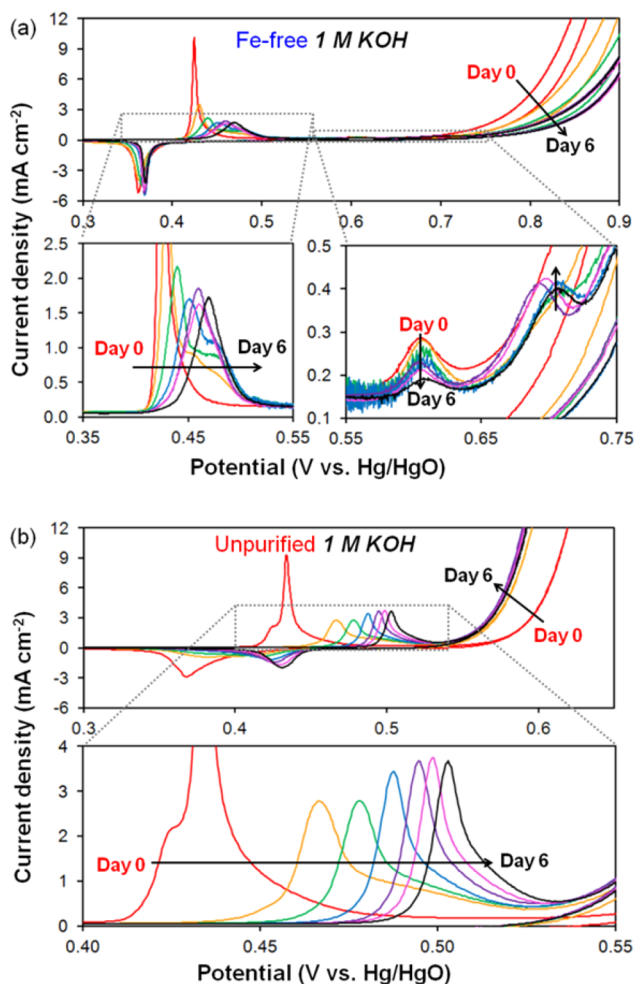
Figure 2. Cyclic voltammograms obtained for \text{Ni}(\text{OH})_2 films deposited on polished Au RDEs. Voltammograms were collected at 10 \text{ mV s}^{-1} and 1600 \text{ rpm} in (a) Fe-free and (b) unpurified 1 \text{ M KOH} after each day of aging in either Fe-free or unpurified 1 \text{ M KOH} , respectively. The oxygen evolution equilibrium potential is 0.306 \text{ V vs Hg/HgO} in 1 \text{ M KOH} .
