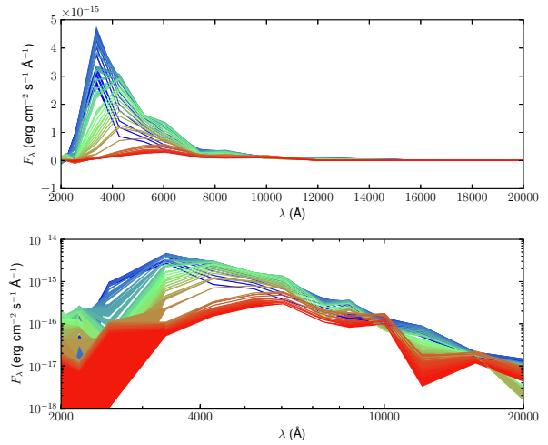
Figure 7. Rest-frame low-resolution SED time series of LSQ12gdj, 1550–23100 Å, constructed from Swift UV + CSP BVri photometry. SED colours show the phase, ranging from blue ( -10 days) to red ( +45 days). Top: linear scale; bottom: log scale. Colored bands represent the 1\sigma confidence region around the mean.
