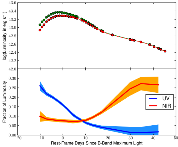
Figure 8. Rest-frame bolometric light curve of LSQ12gdj obtained by integrating the SED of Figure 7. Top: Bolometric light curve 3300–23100 Å (red) and 1550–23100 Å (green) representing the results with and without Swift UV, including Gaussian process regression fit (connecting curves). Bottom: Fraction of bolometric flux bluewards of 3300 Å (“UV”) and redwards of 8800 Å (“NIR”, estimated from a template); the solid curves show the mean behavior, and the lighter bands show the 1\sigma confidence region around the mean.
