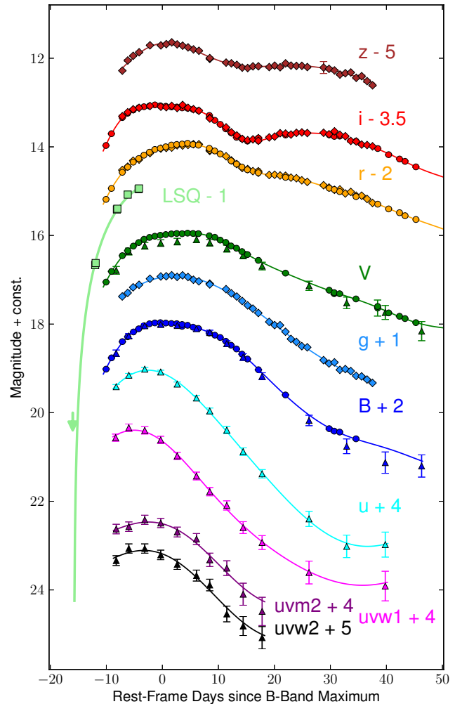
Figure 2. Multi-band light curves of LSQ12gdj. CSP and LCOGT points are shown as circles, Swift points are upward-facing triangles, and LSQ points are squares. Solid curves: Gaussian process regression fit to the data (see Rasmussen & Williams 2006; Scalzo et al. 2014), except LSQ, for which the Arnett (1982) functional form is used (well-approximated by a t^2 rise at early times). Light curve phase is with respect to B -band maximum at MJD 56252.5 (2012 Nov 21.5).
