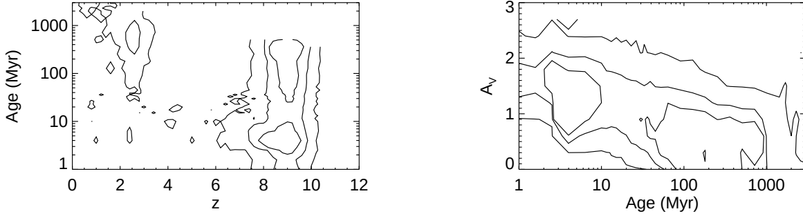
FIG. 3.— Confidence intervals show that a z \sim 9 solution is preferred at the 1\sigma level, while age and extinction are not strongly constrained. Contours are 1, 2, and 3\sigma . On the left hand panel, contours are open because best-fit ages are restricted to be younger than the age of the universe.
