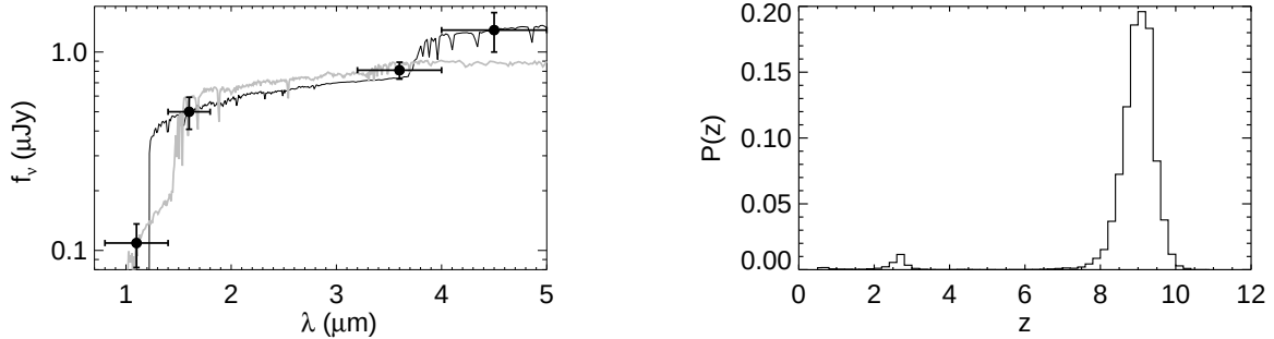
FIG. 2.— Left — The photometry of JD2325+1433 shows two breaks in the spectrum, consistent with the Lyman and Balmer breaks and suggesting a redshift of z \sim 9 . The black curve is the best fit model ( z = 9.0 with an age of 64 Myrs, a constant SFR of 930 M_{\odot} \text{ yr}^{-1} , A_V = 1.0 , M_B = -23.8 , M = 5.4 \times 10^{10} M_{\odot} and Z = 0.2Z_{\odot} ). The grey curve is an alternate, poor fit at z = 2.9 (an instantaneous burst aged 360 Myrs, with A_V = 0.1 , M_B = -21.1 , M = 1.8 \times 10^{10} M_{\odot} and Z = Z_{\odot} ). Right — The results of our Monte Carlo simulation show probability as a function of redshift. More than 96% of solutions lie at z \geq 7 .
