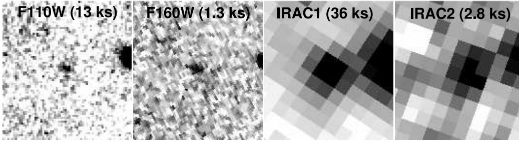
FIG. 1.— Postage stamp images of JD2325+1433 show that it is elongated in the NICMOS images. Images are 6'' on a side. Note that the integration in J_{110} is 10 times longer than in H_{160} , and the integration in IRAC1 ( 3.6 \mu\text{m} ) is 13 times longer than in IRAC2 ( 4.5 \mu\text{m} ), so the galaxy is indeed red in J_{110} - H_{160} , and [3.6] - [4.5] . The coordinates of JD2325+1433 are 23h24m46.52s, 14d32m59s, bootstrapped to the 2MASS frame.
