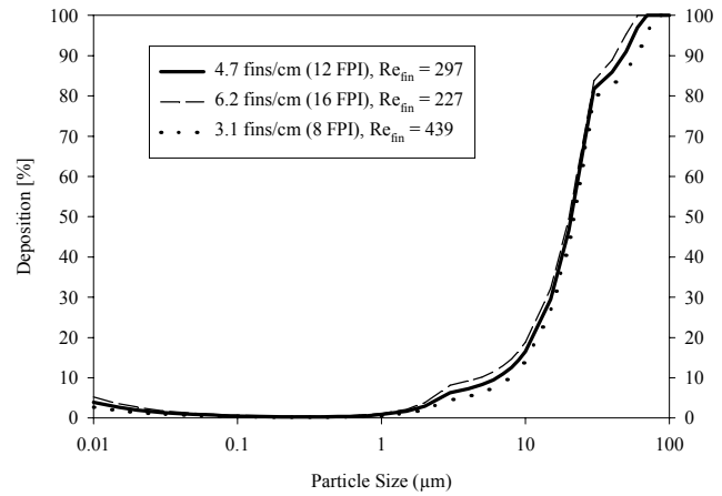
Figure 1: Modeled Deposition as a Function of Fin Spacing for a Bulk Air Velocity of 2 m/s (394 ft/min).
