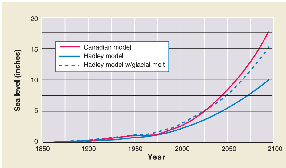
Fig. 7. Projections of sea level rise using the Canadian Climate Center and British Meteorological Office's Hadley global climate models. Solid lines represent changes directly due to increased ocean temperatures; dashed lines add influence of partial melting of Greenland. Estimates to about 2000 are in general agreement with observations. Source: NAST 2000, p. 112.
