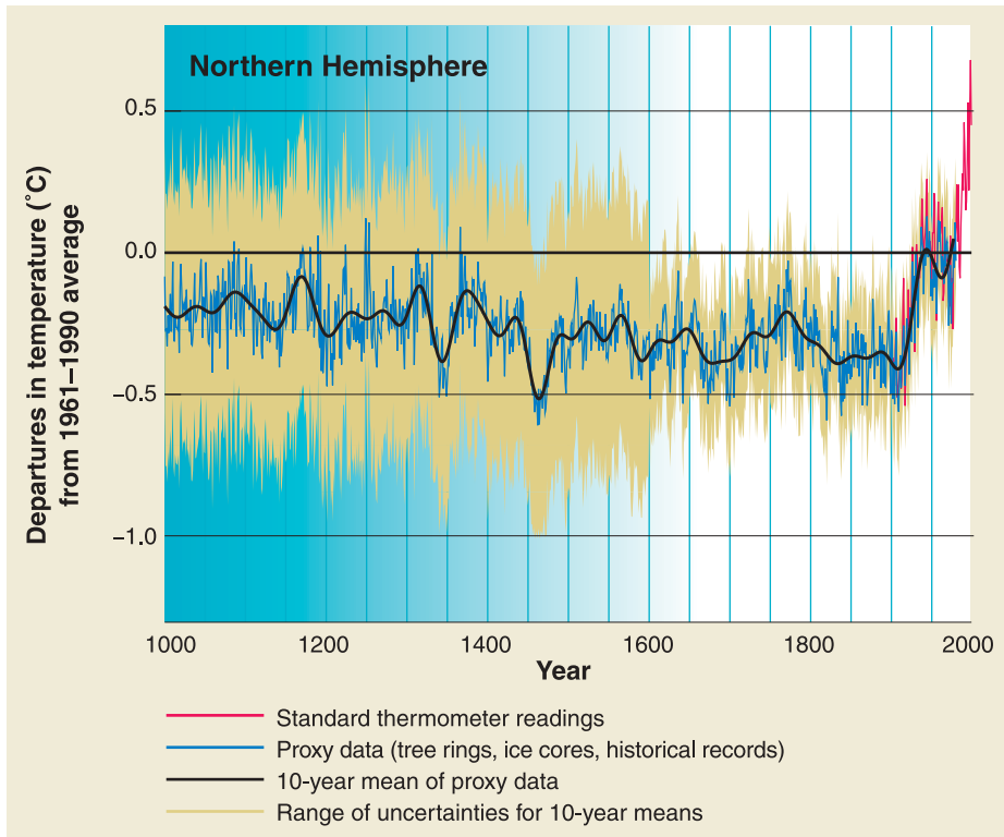
Fig. 3. Northern Hemisphere temperature changes. Source: Houghton et al. 2001, p. 3.
