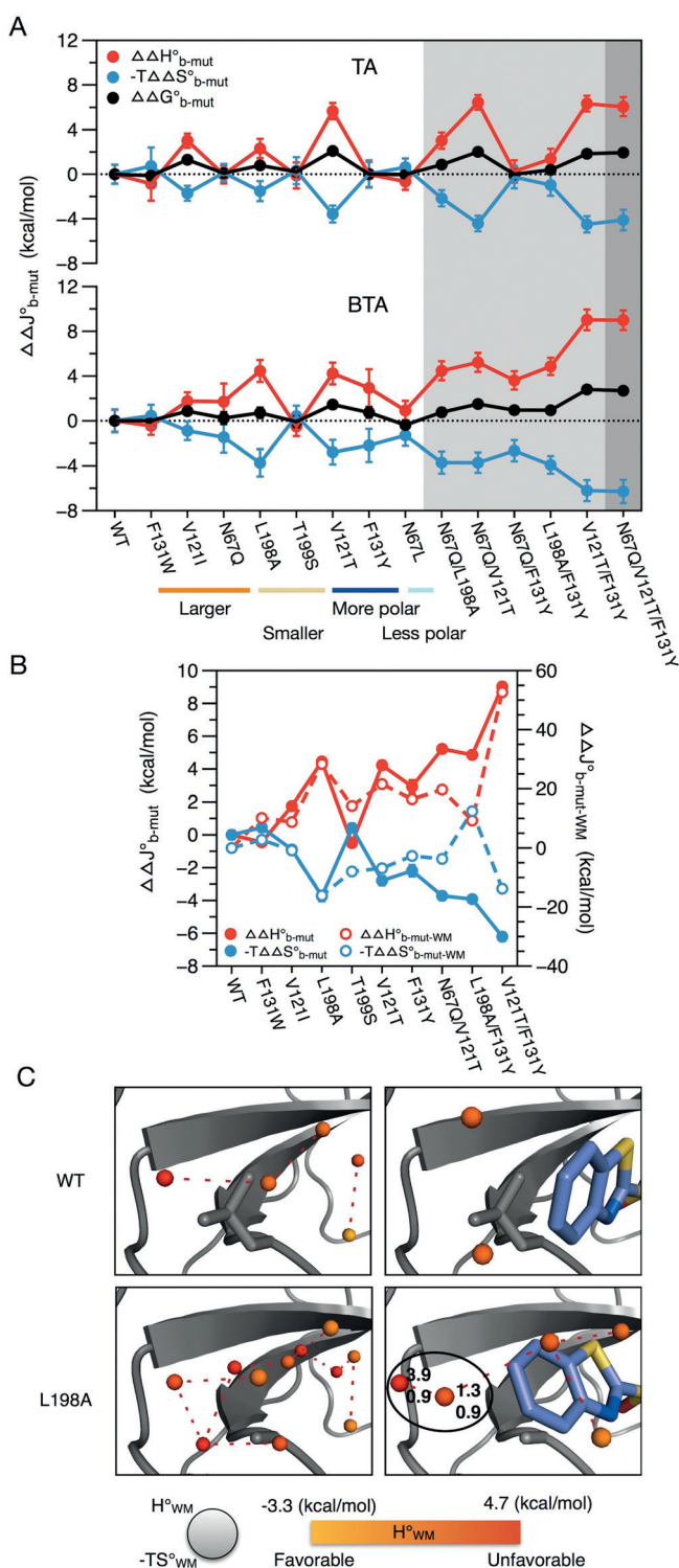
Figure 2. The effect of mutations. A) Differences in the thermodynamic binding parameters of mutants and wild-type HCAII, \Delta\Delta J^{\circ}_{b\text{-mut}} = \Delta J^{\circ}_{b\text{-mutant}} - \Delta J^{\circ}_{b\text{-WT}} . Most mutations cause \Delta H^{\circ}_{b\text{bind}} to become more positive and -\Delta\Delta S^{\circ}_{b\text{bind}} to become more negative in a nearly compensating fashion. B) A comparison of values of mutation-derived changes in enthalpy and entropy of binding determined using ITC (left axis) and WaterMap calculations (right axis). Similar trends between the two sets of parameters suggest that the influence of mutations on the thermodynamic properties of water causes these trends. (Error bars in (A) and (B) represent standard error, n \geq 7 ). C) The influence of L198A on the thermodynamic properties of water. Colors are as follows: Protein (gray) and BTA carbon (purple), nitrogen (blue), and sulfur atoms (yellow). Molecules of water appear as spheres colored according to their enthalpies ( H^{\circ}_{WM} ), relative to bulk water. Plausible hydrogen bonds (intermolecular distances \leq 3 Å) appear as dashed red lines. The leucine-to-alanine mutation strengthens a network of water near the nonpolar wall. During HCAII– BTA association, this network undergoes an enthalpically unfavorable rearrangement (circle). (The circle highlights two enthalpically unfavorable waters). We used X-ray crystal structures for the WaterMap calculations depicted in (B) and (C).
