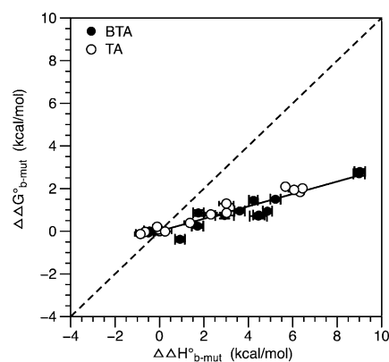
Figure 4. The influence of mutations on binding affinity. Plot showing the influence of mutations on the free energy of binding against their influence on the enthalpy of binding ( \Delta\Delta G_{b\text{-mut}}^{\circ} against \Delta\Delta H_{b\text{-mut}}^{\circ} from Figure 2A). The black line through these points represents a linear fit (slope = 0.29 and R^2 = 0.90 , n \geq 7 ; error bars represent standard error). Mutations that increase the enthalpic cost of binding lower binding affinity (that is, make \Delta G_b^{\circ} more positive).
