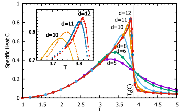
FIG. 3. (Color online). As in Fig. 1 but for the specific heat. Inset: fitting for maxima. Data points in the inset are from the Wolff cluster calculations, while the lines are obtained using non-linear fits with general quartic polynomials of the form y = y_m + a_2(x - x_m)^2 + \dots + a_4(x - x_m)^4 , which give the coordinates of the maximum (x_m, y_m) nearly independent from the rest of the coefficients.
