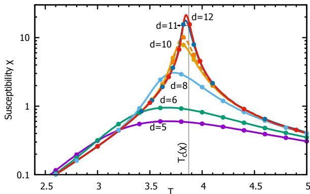
FIG. 4. (Color online). As in Fig. 1 but for the susceptibility \chi(T) , plotted in semi logarithmic scale. The vertical line shows the critical temperature extrapolated from the susceptibility maxima, see Fig. 5.
