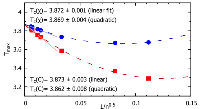
FIG. 5. (Color online). Extrapolation of the specific heat and susceptibility maxima to infinite system size. Red squares (blue circles) show the positions of the specific heat (susceptibility) maxima extracted from the data on Figs. 3 and 4, respectively for graphs of different size, plotted as a function of 1/n^{1/2} , where n is the number of edges in the corresponding graphs, see Tab. I. Solid (dashed) lines are obtained as linear (quadratic) fits to the data, where only the four left-most points were used for the linear fits. This results in the extrapolated critical temperature values as indicated.
