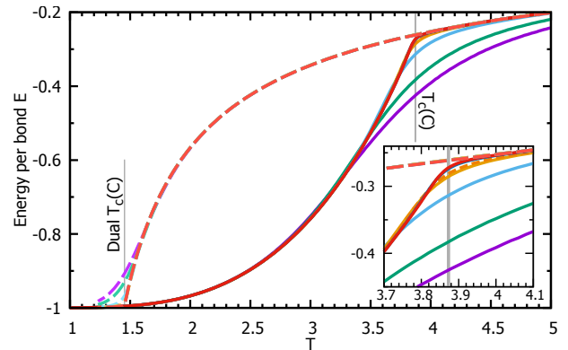
FIG. 2. (Color online). Solid lines: energy per bond from Wolff cluster calculations as a function of temperature, as in Fig. 1. These data are converted with the help of the exact duality (9) to give energies in the dual model (long dashes). With increasing graph sizes, the difference between the original and dual energies decreases above the empirically found T_c(C) (Fig. 5) and below the corresponding Kramers-Wannier dual, T_c^*(C) . Inset: close up of the plots near T_c(C) .
