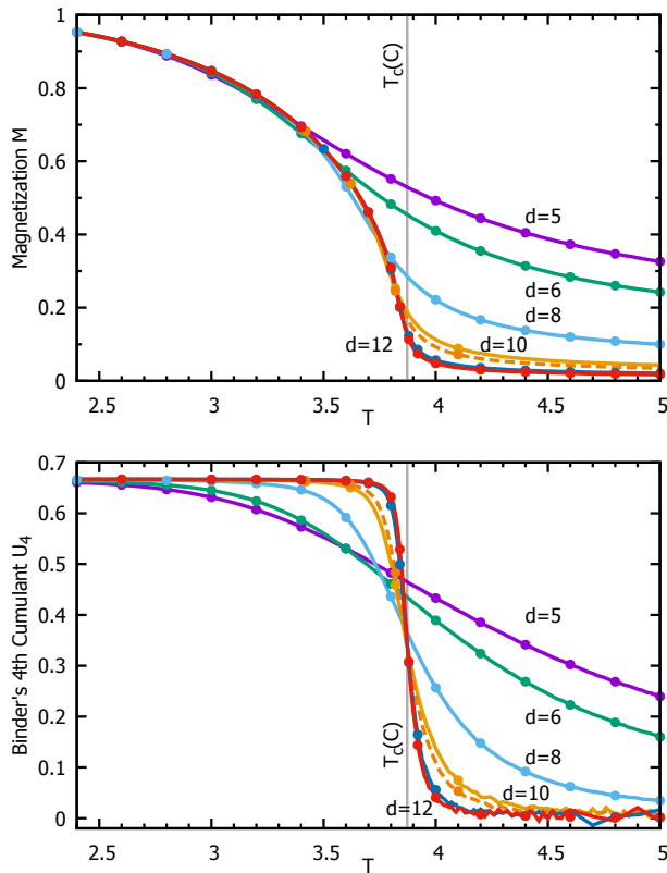
FIG. 1. (Color online) Average magnetization (top) and Binder's fourth cumulant (bottom) as a function of temperature, for transitive graphs listed in Tab. I with minimal distances as indicated. Dashed lines show the data for the larger d = 10 graph. Lines show the data obtained using cluster updates; points show the data from simulations using local Metropolis updates. Vertical line shows the critical temperature T_c(C) extrapolated from the positions of the specific heat maxima, see Fig. 5. While both sets of data do cross near T_c(C) , there is significant drift with increased graph size. In addition, the curves are near parallel which makes reliable extraction of the critical temperature difficult.
