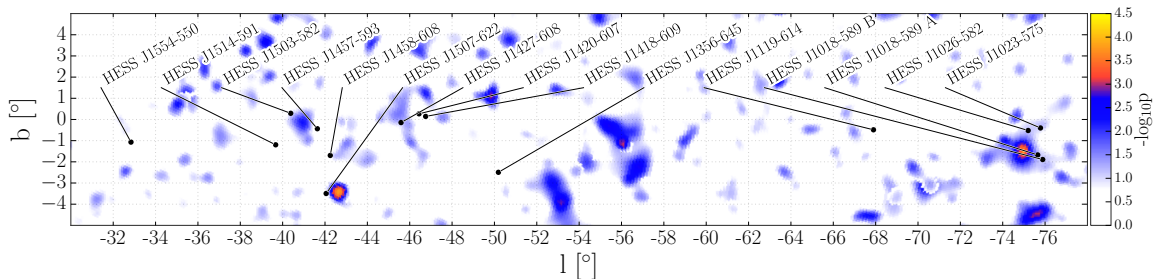
Figure 11. All-sky likelihood scan pre-trial p-value shown in Galactic coordinates for |b| < 5 . The H.E.S.S. sources in the analysis field of view are shown in black.
