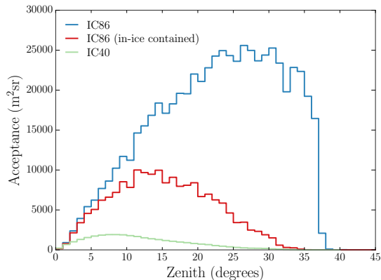
Figure 6. The detector acceptance (effective area integrated over solid angle) as a function of the zenith angle for all gamma rays (blue line), the subset of gamma rays passing through the in-ice array (red line), and for the IC-40 analysis (Aartsen et al. 2013a). The detector response for IC-86 gamma-ray simulations shown here were done using snow heights from October 2012. All three distributions were made assuming an E^{-2.7} gamma-ray spectrum.
