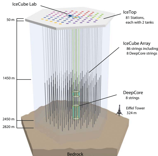
Figure 1. A schematic of the entire IceCube observatory (Aartsen et al. 2017b). The surface array (IceTop) and the in-ice array are shown, along with the in-ice subarray DeepCore.
