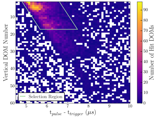
Figure 7. The number of in-ice array hit DOMs binned in vertical DOM number and the hit time ( t_{\text{hit}} ) relative to the IceTop trigger ( t_{\text{trigger}} ), for a collection of experimental events that have no in-ice array HLC hits. The vertical DOM number denotes the position of the hit DOM on its string; larger numbers are on deeper layers of the array. The green box delimits the region within which charge is selected for event classification.
