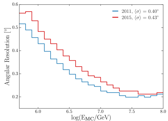
Figure 5. 68% containment intervals of angular resolution to gamma rays from simulation using detector response with snow heights from the first and last year of the data-taking period of the analysis. \langle\sigma\rangle denotes the median angular resolution assuming an E^{-2.0} energy spectrum.
