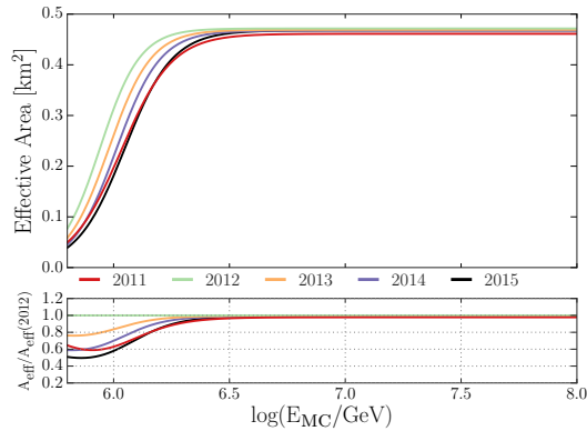
Figure 3. The effective area of IceTop to gamma rays simulated with snow heights from each year of the data-taking period of the analysis. All cuts listed in Section 3 were applied.
