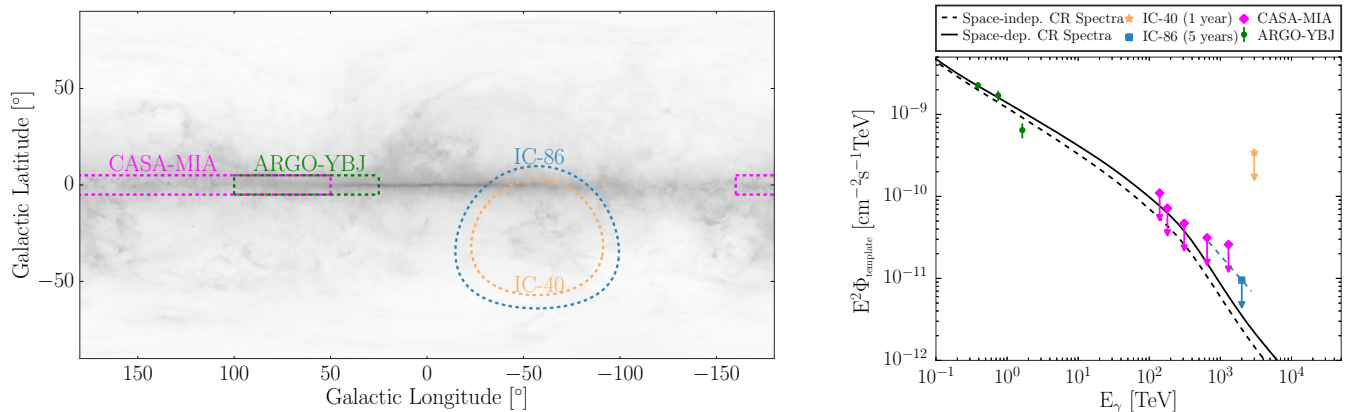
Figure 12. Left: The respective field of views of CASA-MIA (Borione et al. 1998), ARGO-YBJ (Bartoli et al. 2015), IC-40 (Aartsen et al. 2013a), and this analysis overlaid on a map of the \pi^0 decay component of the Fermi-LAT Galactic plane diffuse emission model (Ackermann et al. 2012a). Right: The IceCube 90% confidence level upper limit (IC-86) on the angular-integrated scaled flux from the Galactic plane in our field of view for a spatial distribution of emission given by the \pi^0 decay component of the Fermi-LAT diffuse emission model. The IC-86 upper limit is compared to results from ARGO-YBJ, CASA-MIA, and IC-40, using the scaling defined in Equation 13. Dotted lines show the E^{-3} spectrum, used for obtaining IceCube upper limits, over the energy range containing 5% to 95% events in the final sample. Also shown are, for two models, absorbed flux predictions for the IC-86 field of view calculated by the authors of Lipari & Vernetto (2018) on special request. The two models assume space-independent and space-dependent cosmic-ray spectra throughout the Galaxy, respectively.
