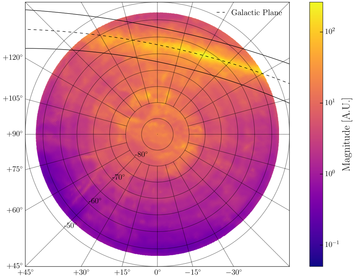
Figure 16. The Fermi-LAT \pi^0 decay spatial template multiplied by the detector acceptance for the data year 2012.
