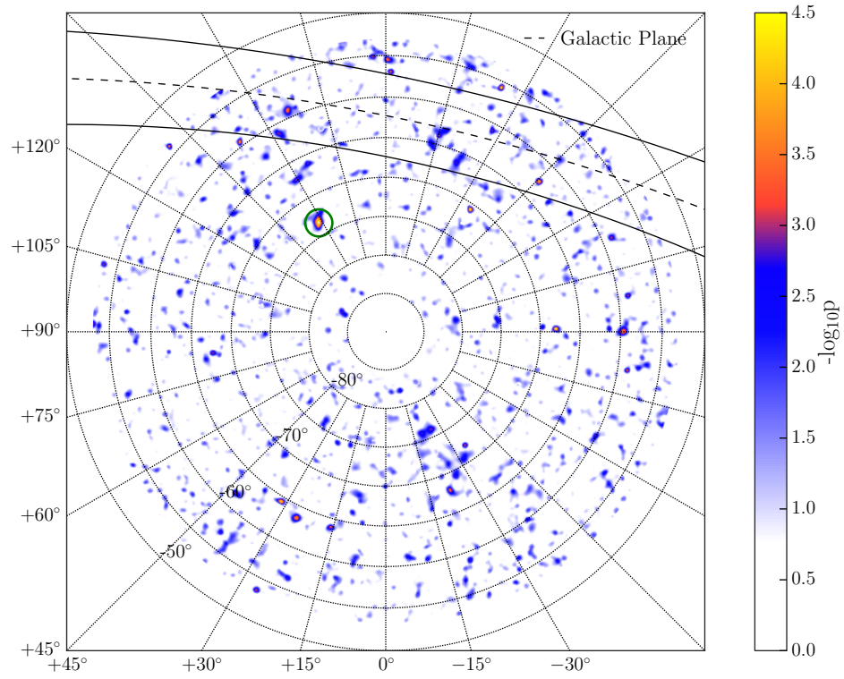
Figure 14. All-sky likelihood scan pre-trial p-values shown projected from the South Pole in equatorial units. The right ascension is labeled along the figure axes, with the interior text denoting declination bands. The green circle highlights the hottest spot in the scan. The Galactic plane region ( <5^\circ in Galactic latitude) is also shown.
