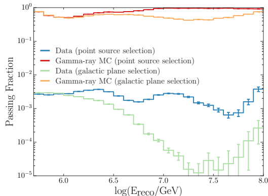
Figure 9. Fraction of events which pass the gamma-hadron discrimination cut for gamma-ray simulation and data (cosmic-ray background) as a function of energy. Both the point source and Galactic plane component event selections are shown.
