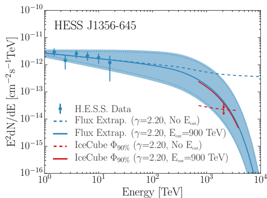
Figure 13. Flux measurements of the source HESS J1356-645 (Abramowski et al. 2011b), along with a power-law spectra with (solid line) and without (dashed line) a 900 TeV cut off in energy, where for both absorption is included for the source distance of 2.4 kpc (Wakely & Horan 2008). For the cut off extrapolation, the shaded region denotes the statistical uncertainty, while the systematic uncertainty is represented by dotted lines. The 90% confidence level upper limit to these flux extrapolations are shown in red.
