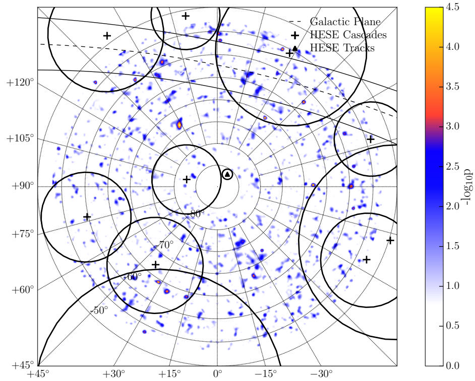
Figure 15. The reconstructed directions and 1\sigma uncertainties of events from the four-year HESE neutrino sample superimposed on the all-sky-scan results.
