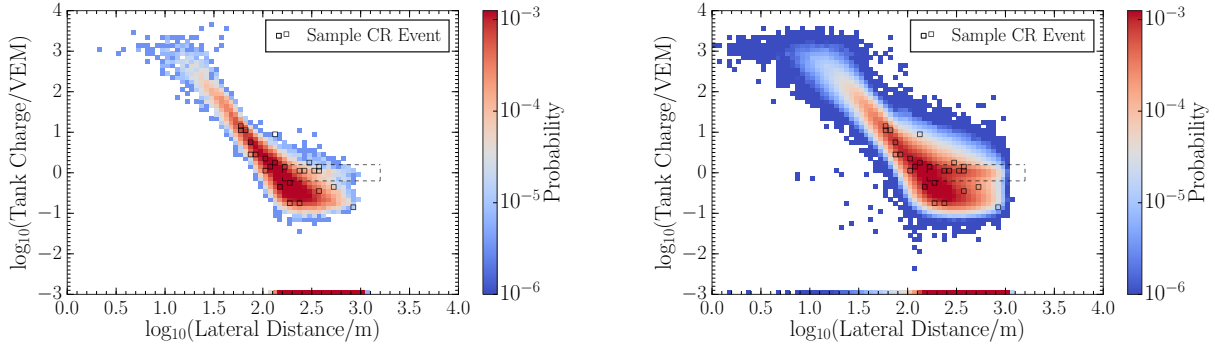
Figure 8. IceTop PDFs, describing the charge distribution as function of the lateral distance of the tank from the shower axis, for simulated gamma-ray (left) and observed cosmic-ray (right) events with 0.3 \leq \log_{10}(S_{125}) < 0.4 and 0.95 \leq \cos(\theta) < 1.0 . Hit tanks for one sample cosmic-ray event are indicated by open boxes on both PDFs and the feature attributed to GeV muons is highlighted using dashed lines.
