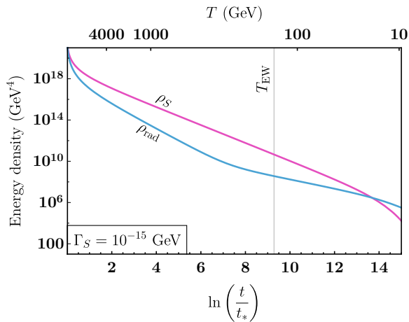
FIG. 1. Energy densities stored in flavon oscillations, \rho_S , and in radiation \rho_{\text{rad}} , with respect to temperature. As a benchmark scenario, it is assumed that \rho_S starts dominating at T_* = 100 TeV and the flavon decay rate is \Gamma_S = 10^{-15} GeV, which corresponds to a decay temperature T_d \simeq 10 GeV. We also show the temperature when the EW sphalerons shut off, T_{\text{EW}} \sim 160 GeV.
