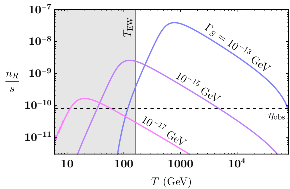
FIG. 3. Right-handed electron asymmetry generated through asymmetric flavon decays for different values of the flavon decay rate \Gamma_S . Observed baryon asymmetry \eta_{\text{obs}} \simeq 8 \times 10^{-11} is shown for reference.
