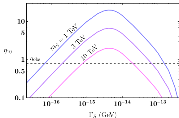
FIG. 4. Baryon asymmetry ( \eta_{10} \equiv \eta_B \times 10^{10} ) of the universe as a function of the flavon decay rate \Gamma_S for different values of the flavon mass m_S . As a benchmark scenario we take the initial flavon asymmetry \eta_S = 1 . The observed baryon asymmetry \eta_{\text{obs}} \simeq 8 \times 10^{-11} is shown for reference.
