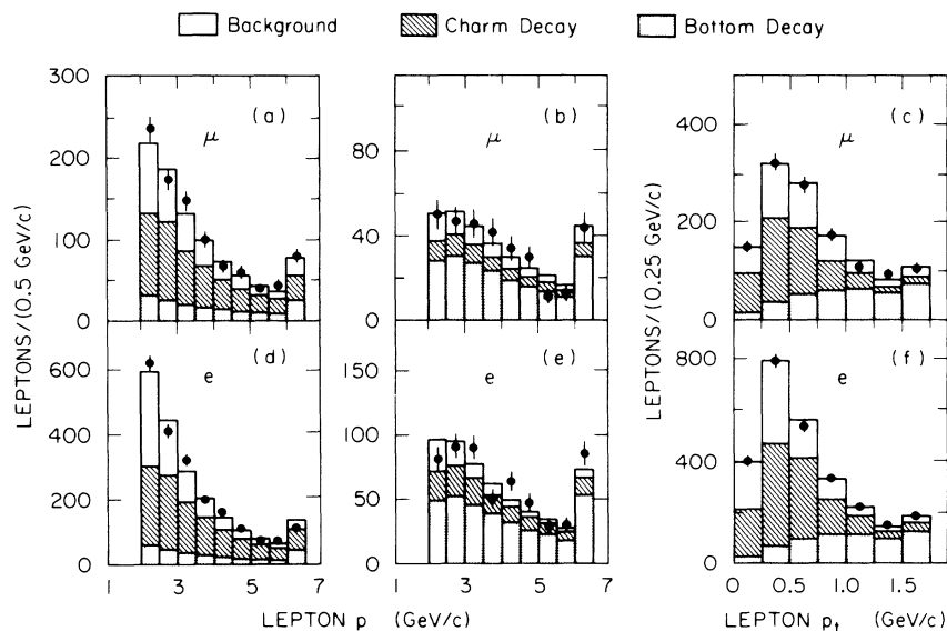
FIG. 1. Lepton momentum and transverse-momentum spectra for the muon and electron samples. The histograms represent the contributions from background, charm decay, and bottom decay (including secondary b decay). The lepton momentum spectra for (a),(d) p_t < 1.0 GeV/c; (b),(e) p_t > 1.0 GeV/c. (c),(f) The lepton transverse-momentum spectra. The highest-momentum bins in (a), (b), (d), and (e) contain all tracks with momenta greater than 6 GeV/c; the highest- p_t bins in (c) and (f) contain all tracks with p_t greater than 1.5 GeV/c. The data points are shown with statistical errors only.
