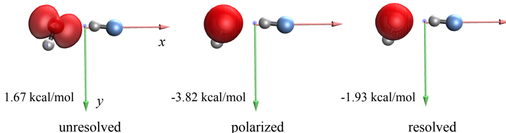
Figure 4: Contour plots of the spin density of the \text{FH}\cdots\bullet\text{OH} complex. All atoms in the complex lie in the xy -plane. The other plotting and computational details are the same as in Fig. 2.
