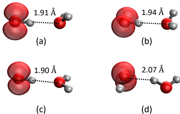
Figure 10: Structures of the \bullet\text{OH}(\text{H}_2\text{O}) complex optimized using \omega\text{B97M-V}/\text{def2-TZVPD} with contour plots of the associated electronic spin densities (with an isovalue of 0.005 a.u.): (a) the global minimum with an {}^2A' electronic state; (b) the structure optimized in the low-lying excited state {}^2A'' ; (c) the transition structure between two equivalent {}^2A' global minima that are symmetric with regard to the plane of the \text{H}_2\text{O} molecule; (d) a local minimum with \bullet\text{OH} serving as the H-bond acceptor. The \text{O}\cdots\text{H} distance for each H-bond is given.
