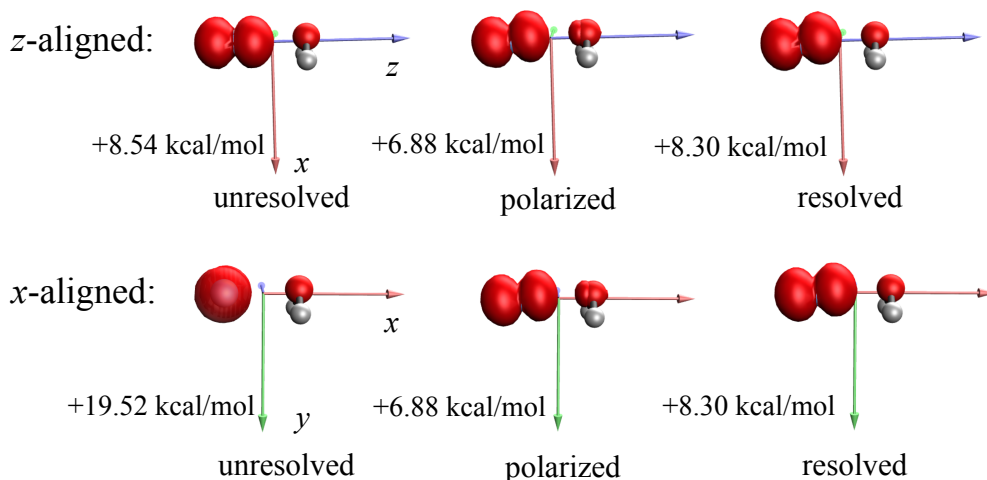
Figure 2: Contour plots (with an isovalue of 0.005 a.u.) of the spin density ( \mathbf{P}_\alpha - \mathbf{P}_\beta ) for the \text{H}_2\text{O} \cdots \text{F}^\bullet complex at different stages of the fragment spin alignment procedure. The \text{F} \cdots \text{O} connection is along the z axis on the upper panels and x axis the lower ones. The leftmost stage (“unresolved”) corresponds to the results obtained directly from fragment SCF calculations, which depend on the orientation of the F orbitals in the lab frame. Orienting the radical electron of \text{F}^\bullet along the \text{F} \cdots \text{O} axis yields an energy increase of 8.5 kcal/mol versus fragments, while a much larger increase of 19.5 kcal/mol occurs when the odd electron is perpendicular. The middle (“polarized”) and rightmost (“resolved”) stages correspond to the spin densities associated with the converged SCF-MI solution and the resulting depolarized fragment orbitals, respectively. The total energy of each intermediate state is evaluated relative to the sum of isolated fragment ( \text{H}_2\text{O} and \text{F}^\bullet ) energies at the M06-2X/def2-TZVPD level of theory.
