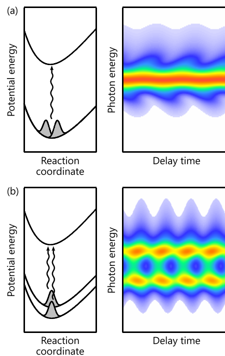
FIG. 2. Probing mechanisms of coherences in tr-XAS. (a) Vibrational coherences induce coherent structural dynamics in chemical systems, which translate to delay-dependent variations in x-ray absorption energies. (b) A coherent superposition of electronic states will lead to characteristic modulation in the absorption amplitude or quantum beats. Adapted with permission from Kobayashi et al. , Phys. Rev. A 101 , 063414 (2020). 16 Copyright 2020 by the American Physical Society.
