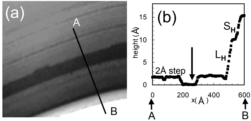
Figure 1. (a) 650 \times 650 \text{ \AA} STM image of the 2-fold Al-Ni-Co surface ( V_s = 1.0\text{V} , I_t = 0.1\text{nA} ). Steps and terraces composed of rows of atoms are visible. (b) Line profile showing steps with heights 4.7 \text{ \AA} ( S_H ), 7.8 \text{ \AA} ( L_H ), and 1.9 \text{ \AA} . The ratio of L_H to S_H is approximately equal to the Golden Mean (1.618), characteristic of aperiodic quasicrystalline structure. The lowest terrace, indicated by the arrow in (b), is a domain where the periodicity along the rows is 8 \text{ \AA} . In the other terraces the periodicity along the rows is 4 \text{ \AA} .
