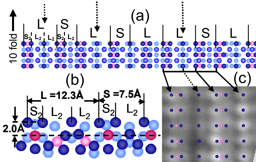
Figure 4. Atomic model of the 2-fold surface derived from the bulk x-ray diffraction model of Takakura et al. (ref. 20). Al is blue and transition metal (Ni, Co) is red. The plane shown here is the one containing only Al atoms, which provides the best fit with the experimental STM images. (a) Top view ( 8 \text{ \AA} \times 90 \text{ \AA} ). There three levels of color of the Al atoms corresponding to relative distances below the surface (dark = top; medium = -0.5 \text{ \AA} , light = -2 \text{ \AA} ). The spacing between Al atoms along the 10 fold direction is 4.1 \text{ \AA} , and the sequence along the 2 fold direction shows the same Fibonacci sequence (LSLSLLSL or S_2L_2L_2S_2L_2S_2L_2S_2L_2S_2L_2S_2L_2S_2L_2S_2L_2S_2L_2S_2L_2S_2L_2 ) as the STM image in Fig. 2c. Dashed arrows mark the positions of local mirror planes. (b) Cross-section showing the atomic arrangement perpendicular to the surface (perpendicular to the 10-fold direction). A transition metal rich layer is visible below ( \sim 2.0 \text{ \AA} lower) the topmost Al one. (c) STM image of section of L and S with the Al sites indicated by blue dots.
