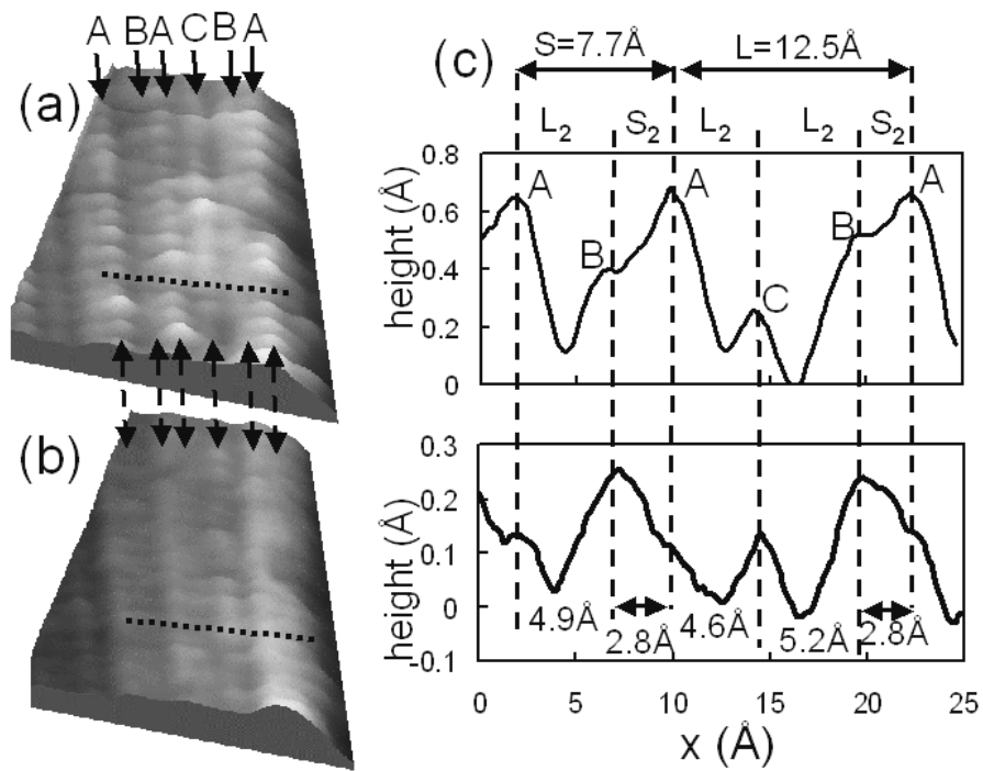
Figure 3. STM images of the same area acquired at positive and negative bias. (a) V_s = +1.2\text{V} , I = 0.1\text{nA} (b) V_s = -1.2\text{V} , I = 0.1\text{nA} . (c) Line profiles across the dashed lines in (a) and (b) reveal three electronically different atomic rows, labelled A, B, and C.
