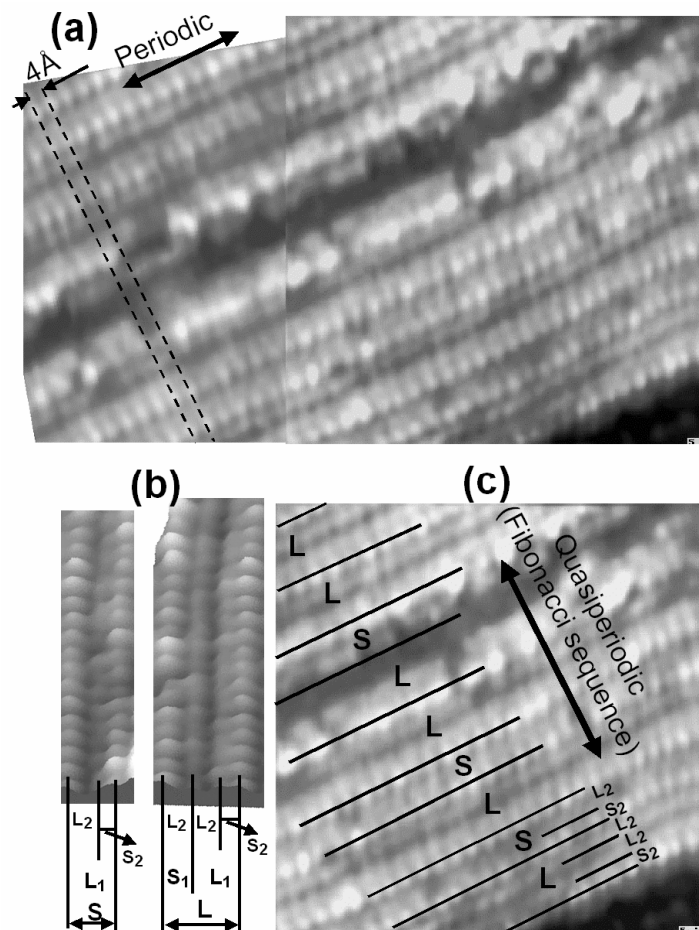
Figure 2. (a) Collage of STM images ( 145 \text{ \AA} \times 90 \text{ \AA} ) of two contiguous regions in the 2-fold Al-Ni-Co surface. The terraces are made of rows of periodically arranged atoms ( 4 \text{ \AA} ) along the ten fold direction and separated by distances L and S. (b) Expanded view showing the interior in the L and S sections. L contains two atomic rows, separated by L_2 and S_2 distances. S contains one row, at distances of L_2 and S_2 from the boundary. (c) The sequence of L and S spacings between rows follows a Fibonacci sequence. The trench in the center of (a) and (c) is due to a missing L+S section. The complete Fibonacci sequence of LSLSLLSLLS is visible in 2a.
