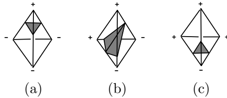
Figure 5 Two cases to be considered for an isosurface passing through a tetrahedron: (a) and (c) are symmetrical cases of a one-triangle configuration, and (b) shows a two-triangle configuration.
