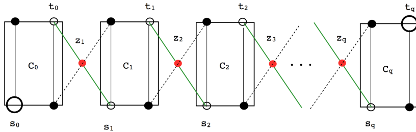
Figure 1.4: An accordion-like structure illustrating the proof of the rematching lemma. Unfilled circles represent vertices left unmatched by inductively invoking the lemma on each C_k . Solid black, vertical lines represent the matching M while solid green, diagonal lines represent the newly matched pairs of M' . Dashed, diagonal lines illustrate the additional length i shortest paths passing through each z_k . This accordion-like structure recursively takes place within each C_k . Note that s_0 = \hat{s} and t_q = \hat{t} .
