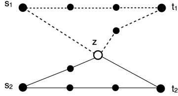
Figure 1.3: Dashed and solid lines represent the shortest paths from s_1 to t_1 and s_2 to t_2 , respectively. Let S = \{s_1, s_2\} and T = \{t_1, t_2\} . (S, T) is a 3-consistent pair since d(s_1, t_1) = d(s_2, t_2) = 3 . Observe that d(s_1, t_2) = 2 and d(s_2, t_1) = 4 and so the paths from s_1 to t_2 and from s_2 to t_1 are not in \mathcal{P}^{(S, T)} ; however these paths will be present in the cover graph G^{(S, T)} . Furthermore, the fact that z lies at step 1 along a length 3 shortest path from s_1 to t_1 and at step 2 along a length 3 shortest path from s_2 to t_2 shows that G^{(S, T)} is not a 3-layered DAG and so (S, T) is not 3-good. However, it is instructive to note that M^* would match s_1 to t_2 and s_2 to t_1 since this maximizes \Psi(\cdot) .
