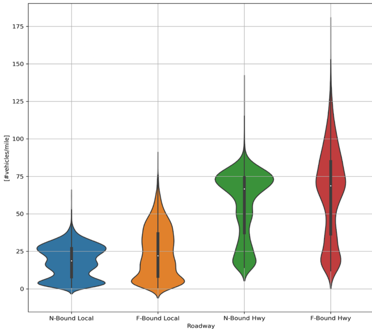
Figure 6. Traffic density (vehicles/mile) distributions for segments (left-to-right): local 9 (blue, eastbound), local 2 (orange, westbound), freeway 4 (green, southbound), and freeway 1 (red, northbound). The median value is indicated by the central white dots of the inner box plots.
