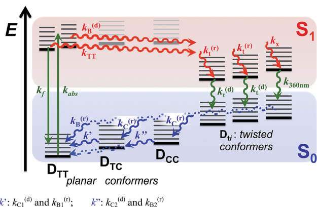
Scheme 4 Excited- and ground-state dynamics of THIA as determined from transient-absorption kinetics. k^{\cdot} : k_{\text{C}}^{(\text{d})} and k_{\text{B}}^{(\text{r})} , k^{\cdot\cdot} : k_{\text{C}}^{(\text{d})} and k_{\text{B}}^{(\text{r})} .
