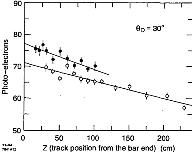
Figure 6: Track position dependence of the photo-electron yield at a dip angle \theta_D = 30^\circ . The solid circles are measurements with the 120 cm long bar and the open circles are with the 240 cm long bar. The solid lines are exponential fits to the data with an effective attenuation rate of 11.2 %/m and 8.7 %/m, respectively.
