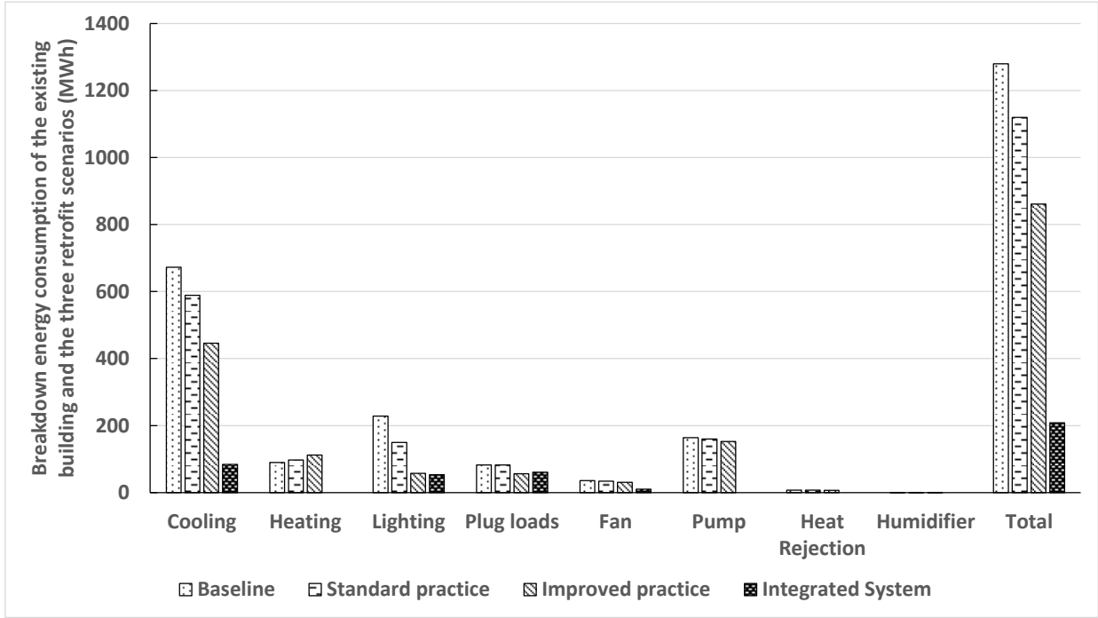
Figure 8. A comparison of the breakdown of electricity consumption between the existing building, the Standard Practice, Improved Practice and the Integrated System retrofit approaches.
