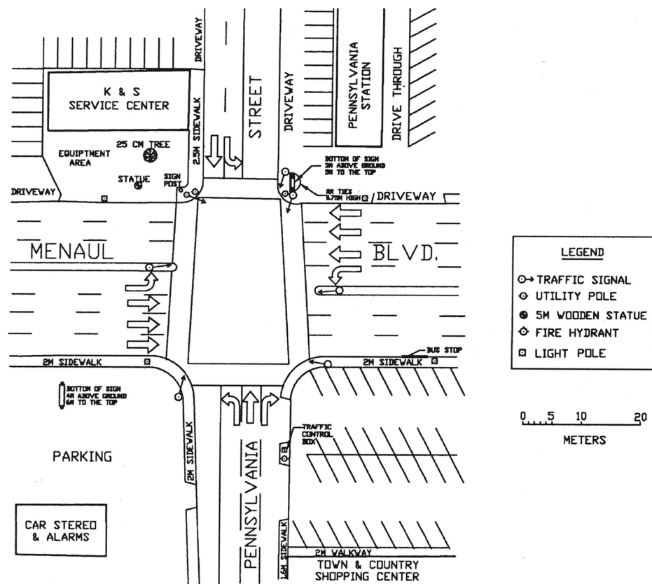
Fig. 9-6—Condition Diagram
