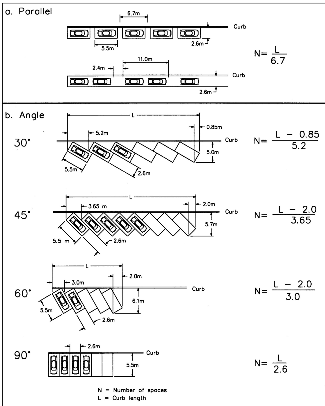
Fig. 23-1—Curb Parking Spaces at Various Angles
