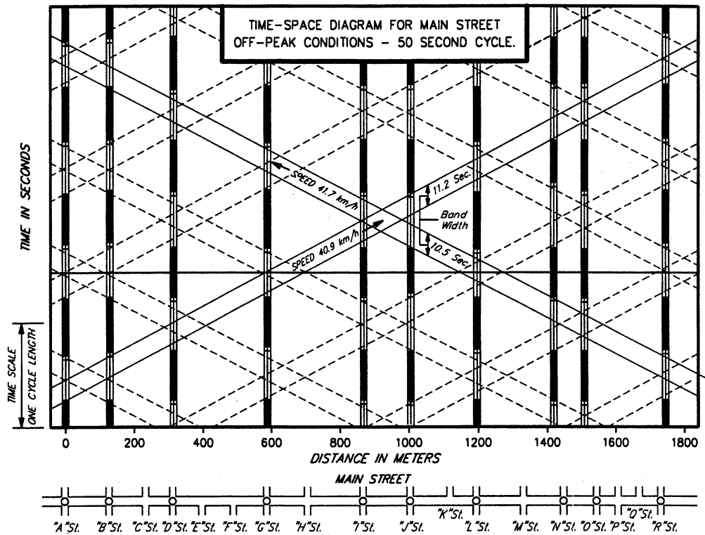
Fig. 16-1—Time-Space Diagram Treating Both Directions of Traffic Equally
