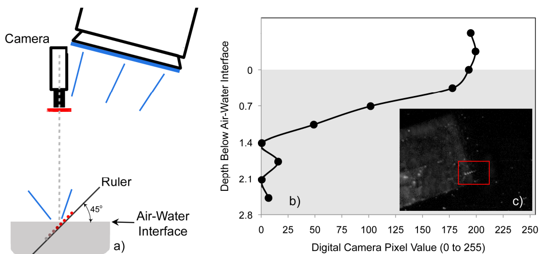
Figure 3. Measurements quantifying the attenuation of microsphere visibility in the dyed channel water. In a) the measurement method is shown graphically. In b) the brightness values of the microspheres, obtained the grayscale values from the CCD pixels corresponding to the locations of the microspheres on the ruler, are shown to decrease with depth and approach zero after ~1 mm. In c) the raw camera image is shown, where the ruler descends into the water from the left and the glued microspheres are clustered close together in a short line, within the red rectangle.
