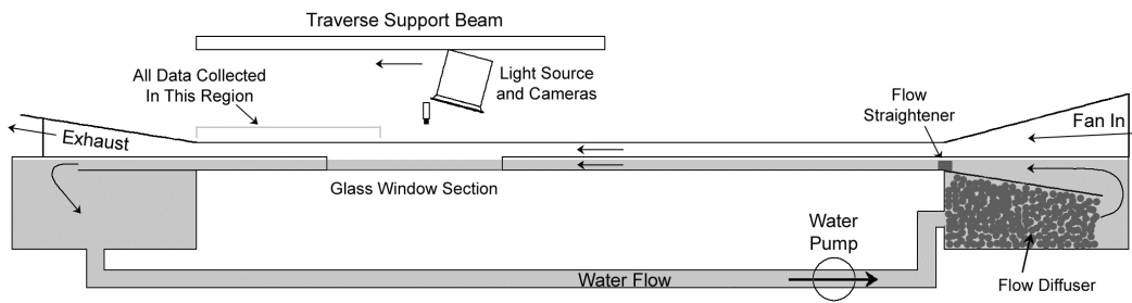
Figure1. The wind wave channel in which the experiments were performed. The water level is denoted by the shade of gray. The top half of the channel was constructed of clear acrylic plastic. The bottom half was stainless steel. The large tanks were made of HDPE plastic. A glass window replaced this steel over a 1.7 meter section of the channel, and allowed viewing of the flow from the sides and bottom. In the upstream tank a pile of random packing was placed for use in different experiments, not reported here, but this random packing acted coincidentally as a good flow diffuser.
