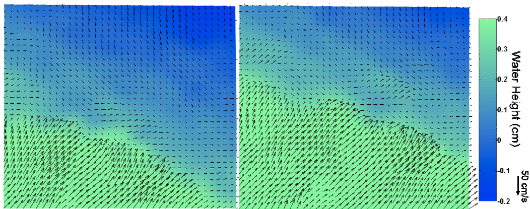
Figure 5. Results from the 3D-IPIV method for two time slices. The image on the right was collected 0.016 seconds after the image on the left. The velocity vectors are corrected so as to correspond to a contorted surface. The color scale on the right gives the height of the air-water surface relative to the mean height. The 50 cm/s vector on the right gives the scale for the velocity vectors. A microscale breaking wave is seen moving up and to the right. Capillary waves populate the face of the wave.
