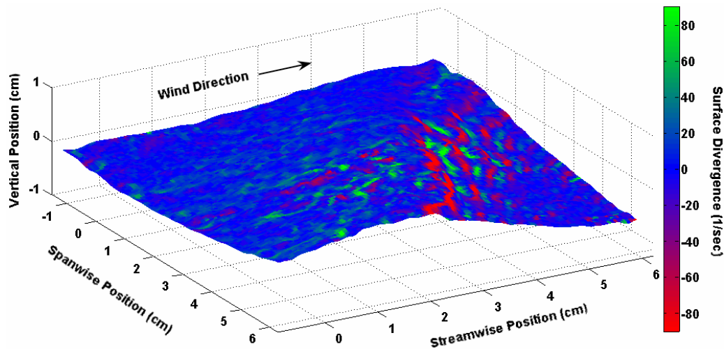
Figure 6. A three dimensional image of surface divergence on a microscale breaking wave. Upwelling is seen behind the wave. Bands of alternating convergence and divergence are seen on the face of the wave, due to capillary waves and also due to the spilling region of the breaking wave.
