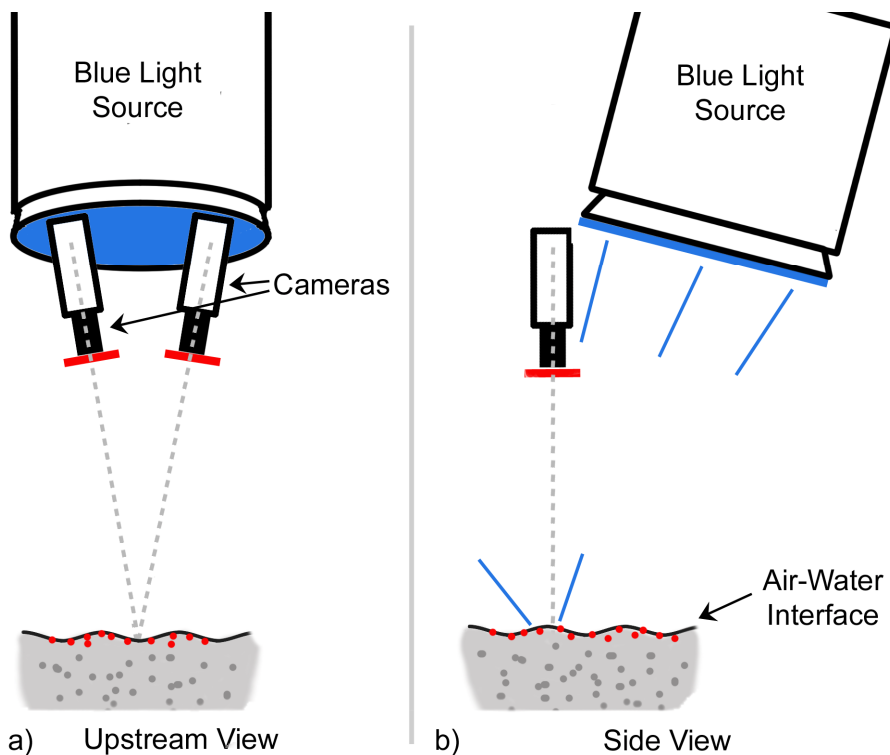
Figure 2. The new 3D-IPIV technique is shown from two angles. In a) the view is looking upstream. In b) the view is from the side as in Figure 1. The water is dyed strongly black. The fluorescent microsphere flow tracers are seen to fluoresce red when they are near the air-water interface, but remain invisible when they are deeper than 1mm in the water phase.
