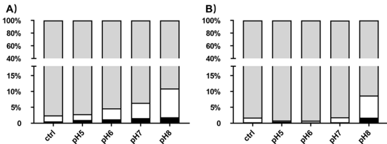
Figure 6. O -Acetyl migration on OAc-Sia-containing sialoglycans. Neu5,9Ac 2 α3Galβ3GlcNAcβProNH 2 ( A ) and Neu5,9Ac 2 α3Galβ4GlcNAcβProNH 2 ( B ) at a different pH by comparing the composition of Neu5,9Ac 2 (gray columns), Neu5,8Ac 2 (white columns), and Neu5,7Ac 2 (black columns) released by sialidase treatment before the low temperature DMB-HPLC analysis.
