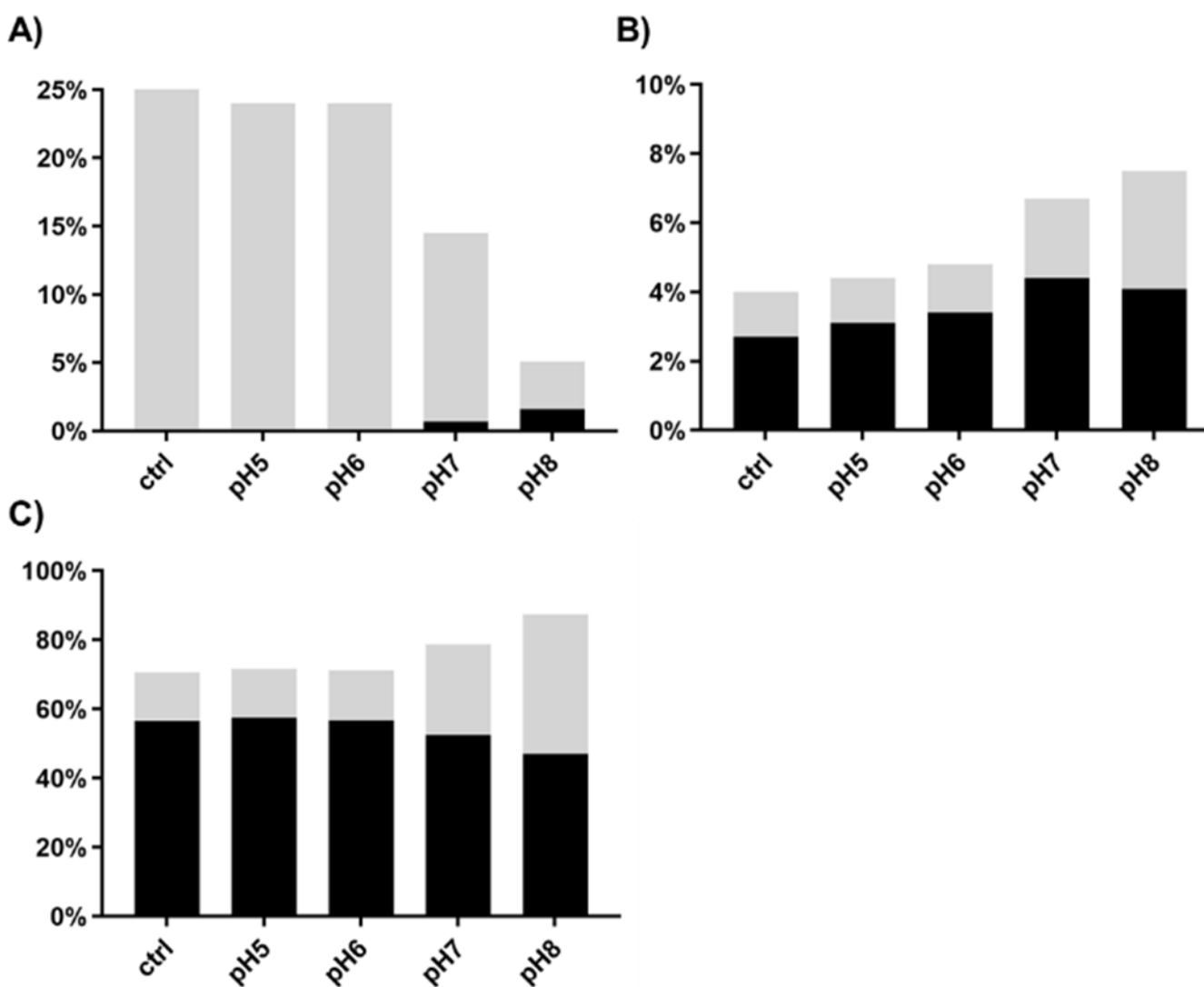
Figure 5. Concurrent interconversion between Neu5,7Ac 2 and Neu5,9Ac 2 at neutral or slightly basic pH.
