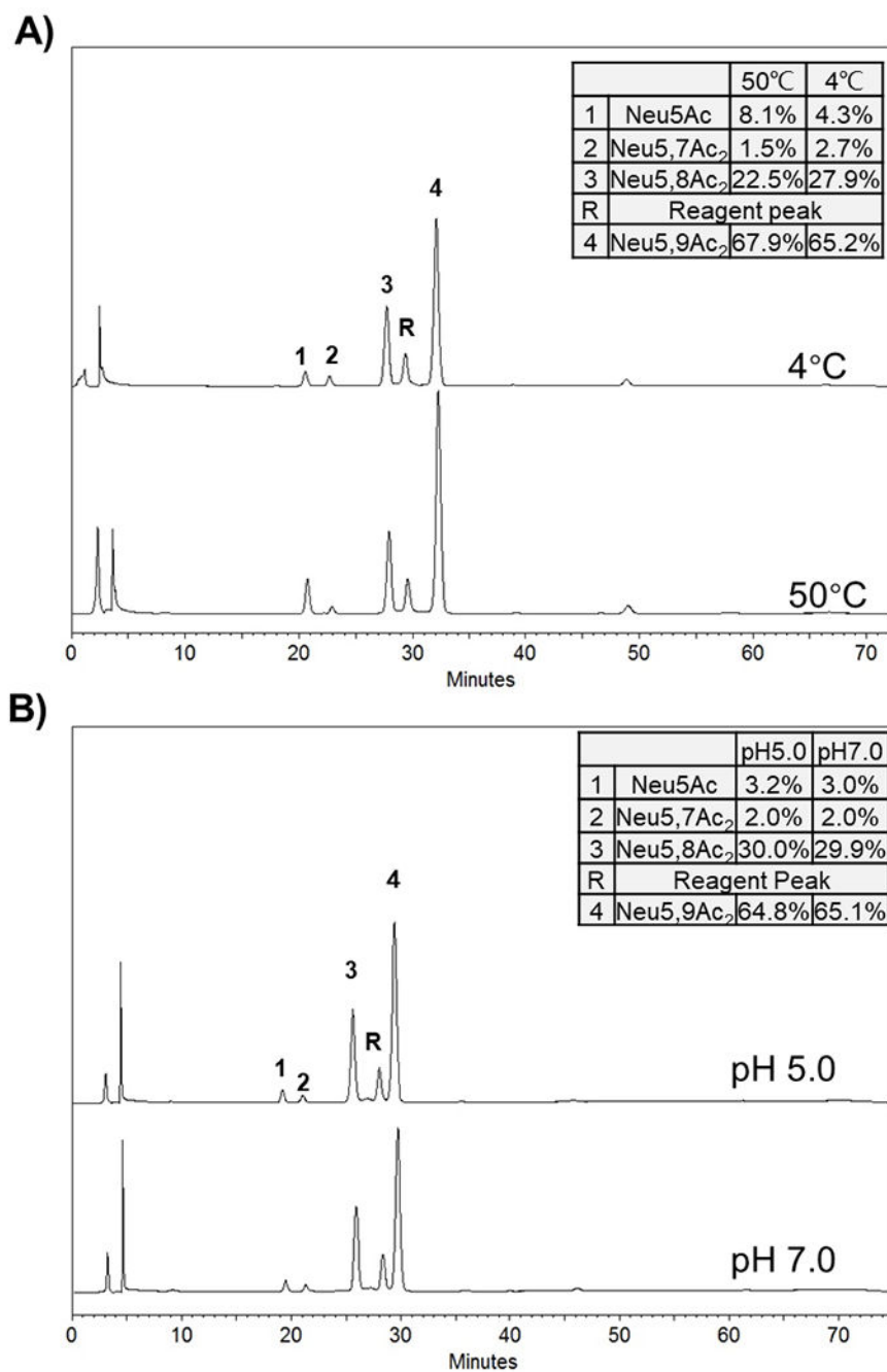
Figure 2. Comparison of DMB derivatization-HPLC analysis methods for quantification of OAc-Sias.
