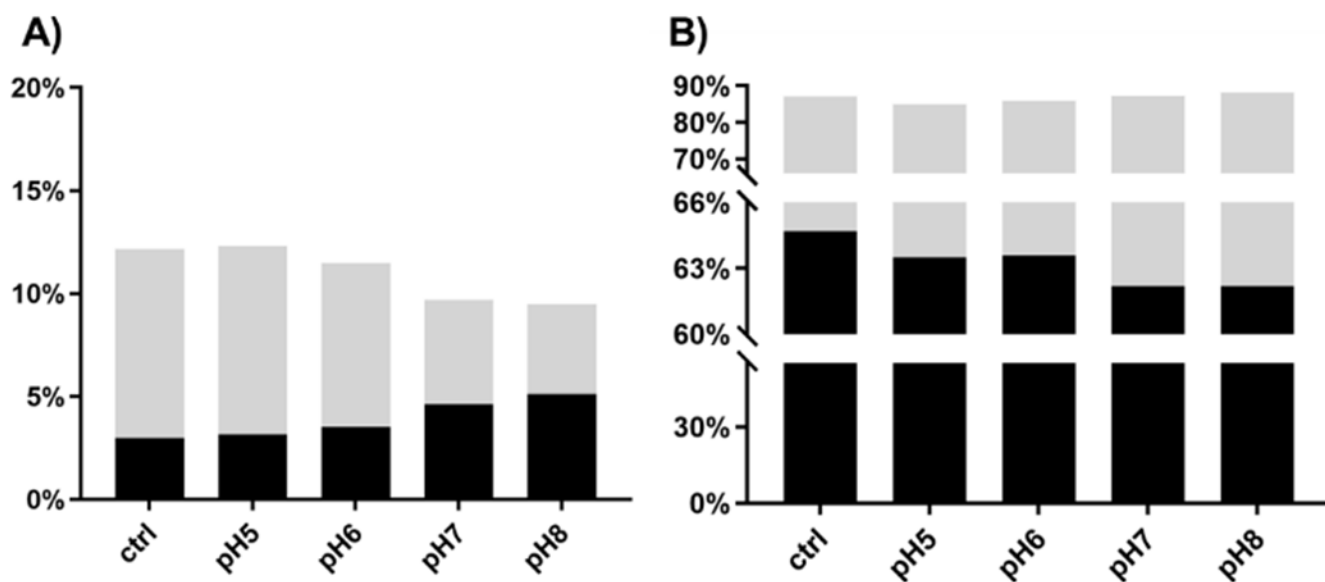
Figure 4. Concurrent interconversion between Neu5,8Ac 2 and Neu5,9Ac 2 at neutral or slightly basic pH.
