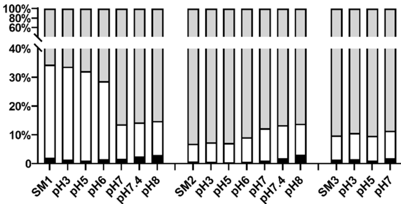
Figure 3. O -Acetyl migration in OAc-Sia monosaccharide samples.
