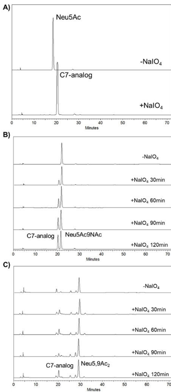
Figure 8. DMB-HPLC assay results of sialoglycan Sia \alpha 3Gal \beta 3(Fuca4)GlcNAc \beta ProNH 2 containing Neu5Ac (A), Neu5Ac9NAc (B), or Neu5,9Ac 2 (C) treated with 6 mM NaIO 4 at pH 6.5, 20 °C, for 30–120 min, followed by sodium borohydride (30 mM) reduction at 20 °C for 20 min, and acetic acid (2 M) releasing of Sias at 80 °C for 1 h.
