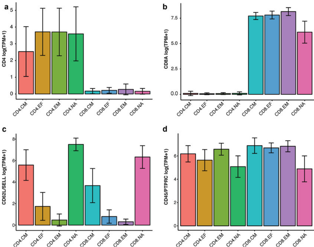
Fig. 4 Expression of known T cell markers (a–d). Illustrative barplots showing the expression (average \pm SD log(TPM + 1)) of key marker genes across the 8 subsets. (a) CD4 , gene encoding for CD4 co-receptor. (b) CD8A , gene encoding the alpha-subunit of the CD8 co-receptor. (c) SELL , gene encoding the lymph node homing receptor CD62L, expressed predominantly on circulating T cells. (d) PTPRC , gene encoding the CD45 antigen, expressed on all T cells
