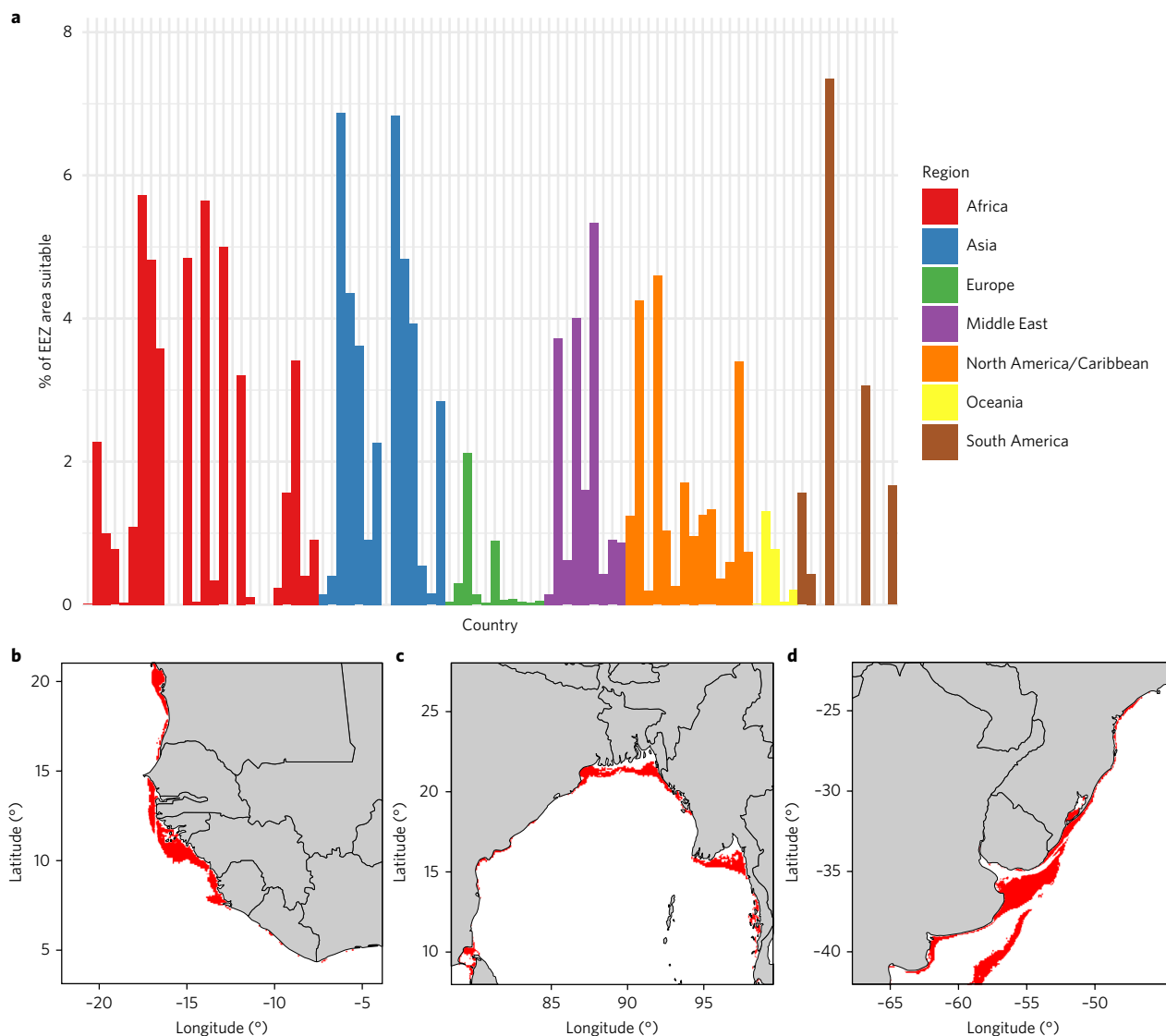
Fig. 2 | Potential growing area for bivalves by country. a , Percentage of each country's exclusive economic zone (EEZ) that has potentially suitable growing conditions for bivalves and no known conflicting uses. Each bar represents a single country grouped by region. b–d Potential bivalve growing areas (red) centred on Guinea ( b ), Bangladesh ( c ) and Uruguay ( d ). These are the countries with the highest percentage suitable areas for bivalves in Africa, Asia and South America, respectively. More detail is provided in Supplementary Fig. 7.
