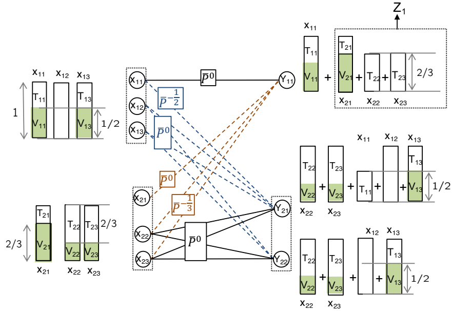
Figure 4.3: Equivalent channel and signal levels at each receiving antenna, where the value on each link is equal to its channel strength level.
