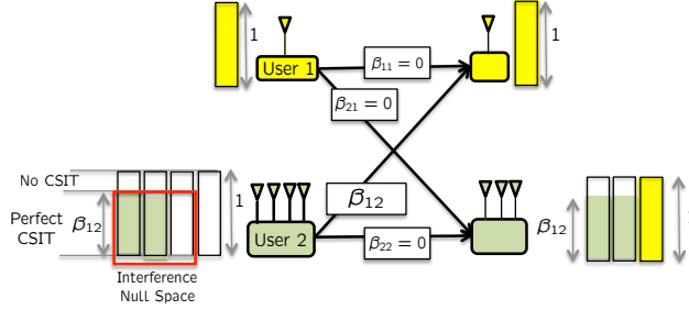
Figure 3.1: (M_1, M_2, N_1, N_2) = (1, 4, 1, 3) , (d_1, d_2) = (1, 2\beta_{12}) .
