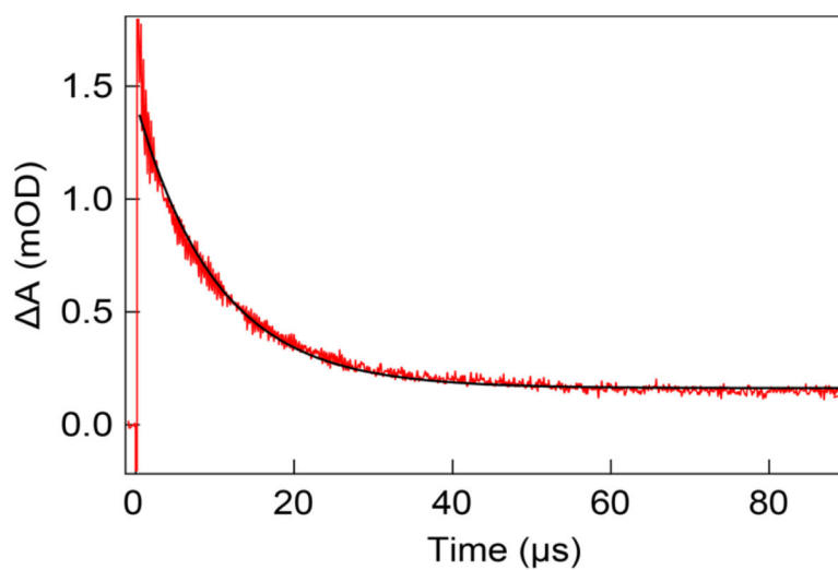
Figure 5. Transient absorption kinetics of 2,3,6-F 3 Y 356 • decay (red) in the presence of C 439 U \alpha_2 , substrate and effector in spectroscopy buffer and associated monoexponential fit. Data represents the average of three independent trials and fit is displayed for illustrative purposes.
