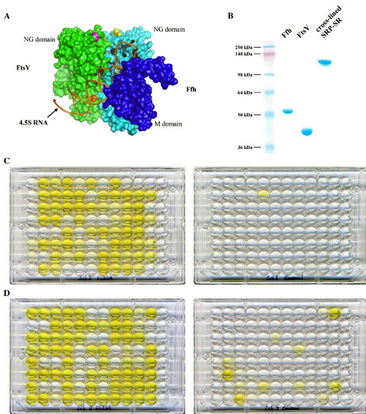
Fig. 1. Panning for scFvs specific for SRP-SR. (A) 3D model of SRP-SR complex showing the spatial relations of Ffh, FtsY and 4.5S RNA. (B) SDS-PAGE analysis of cross-linked SRP-SR. (C) Monoclonal ELISA plate of Tomlinson I library (left) and its control (right). (D) Monoclonal ELISA plate of Tomlinson J library (left) and its control (right).
