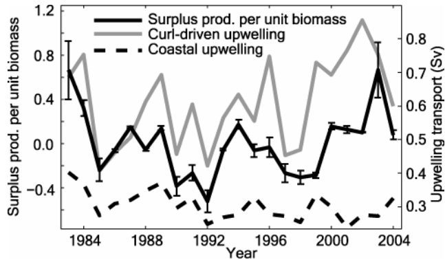
Fig. 5. Upwelling and surplus production per unit biomass of Pacific sardine. Curl-driven upwelling from May-July showed the highest correlation with surplus production per unit biomass ( r = 0.62 , p < 0.005 , n = 22 ). Coastal upwelling during the same period was not significantly correlated with production ( r = 0.40 , p = 0.067 , n = 22 ). Error bars are \pm one standard deviation of the sardine production estimates.
