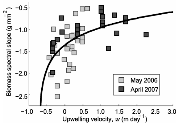
510 Fig. 2. Relationship between zooplankton size and upwelling rate. This relationship is modeled using a logarithmic function ( r^2 = 0.32 , p < 0.001 , n = 51 , y = 0.46 \cdot \ln(x + 0.71) - 1.20 ). The mean 90% confidence interval around the slopes of the linear least-squares fits to the biomass spectra is \pm 0.71 \text{ g mm}^{-2} .
