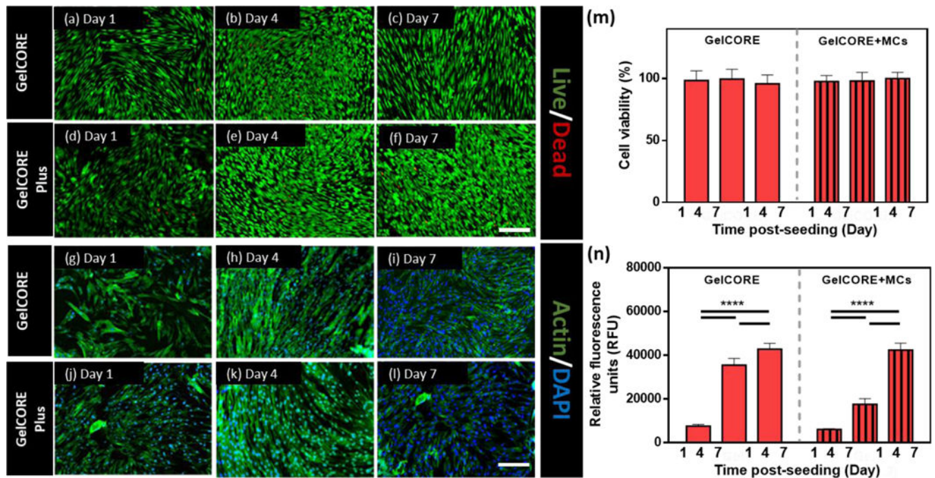
Figure 6. In vitro cytocompatibility of GelCORE+MCs bioadhesive:
