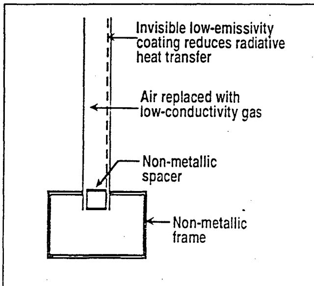
Figure 1. State-of-the-Art Window Technologies
