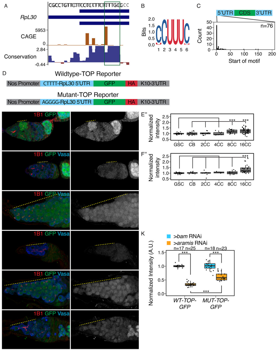
Figure 6. Ais regulated mRNAs contain a TOP motif.
