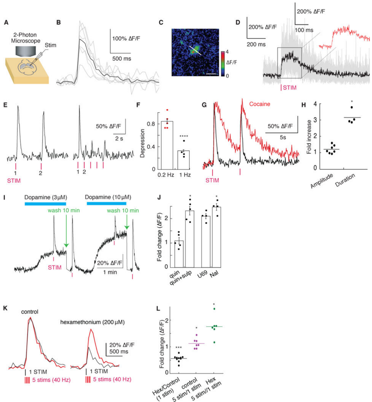
Fig. 2. Imaging electrically evoked and pharmacologically modulated dopamine release in acute dorsal striatum slices
