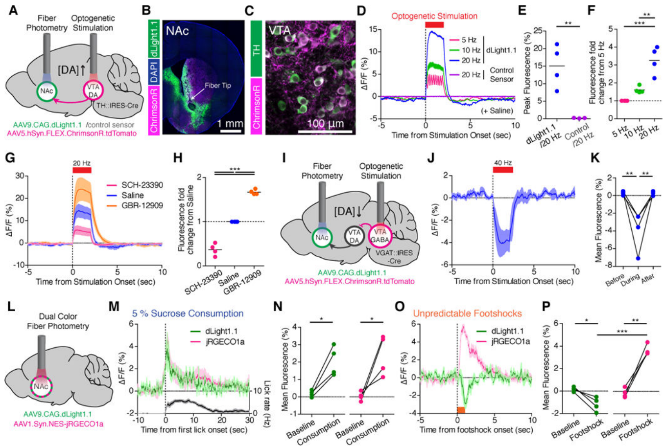
Fig. 3. Deep brain imaging of DA release triggered by optogenetic stimulation and combined with calcium imaging in freely behaving mice (A) Schematics showing fiber photometry recording of dLight1.1 or control sensor in the NAC while stimulating VTA DA neurons by optogenetics. (B) Expression of dLight1.1 in the NAC around fiber tip location and ChrimsonR expressing axons from midbrain. (C) ChrimsonR-expressing TH + DA neurons in the VTA. (D) Averaged fluorescence increase in response to optogenetic stimuli (n = 5 mice) (E) Quantification of peak fluorescence at 20Hz. (F) Fluorescence fold changes relative to 5Hz. (G–H) Optogenetically induced fluorescence increase of dLight1.1 after systemic administration of saline, D1 antagonist (SCH-23390, 0.25 mg/kg) and DA reuptake inhibitor (GBR-12909, 10 mg/kg) (n = 5 mice). (I) Schematics showing fiber photometry recording of dLight1.1 in the NAC and optogenetic stimulation of VTA GABA neurons that inhibits VTA DA neurons. (J–K) Averaged fluorescence decrease in response to optogenetic stimulation at 40 Hz (n = 4 mice) and mean fluorescence quantified in K. (L–P) Dual-color fiber photometry recording of DA release with dLight1.1 and local neuronal activity with jRGECO1a. (M–N) Increase of dLight1.1 (green) and jRGECO1a (magenta) fluorescence during 5% sucrose consumption with lick rate (black, n = 5 mice). Mean fluorescence was quantified in (N). (O–P) Fluorescence decrease in dLight1.1 (green) and increase in jRGECO1a (red) during unpredictable footshock delivery (0.6 mA for 1 sec, n = 5 mice). Mean fluorescence was quantified in (P). Data shown are means ± SEM. Significance was calculated by means of paired or unpaired t
