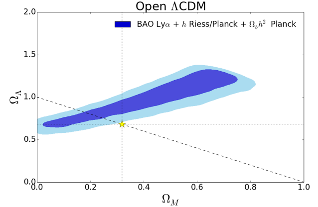
Fig. 14. Constraints on the \Omega \Lambda CDM parameters (\Omega_{\Lambda}, \Omega_M) based on the autocorrelation contours of Fig. 13. The contours show 68.3% and 95.5% confidence levels. The Planck value of \Omega_B h^2 is assumed together with a Gaussian prior for H_0 = 70.6 \pm 3.2 \text{ km s}^{-1} \text{ Mpc}^{-1} . The yellow star is the Planck \Lambda CDM measurement, the dashed line corresponds to a flat Universe.
