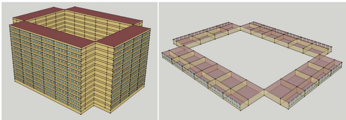
Figure 4. Building model and floor geometry.
