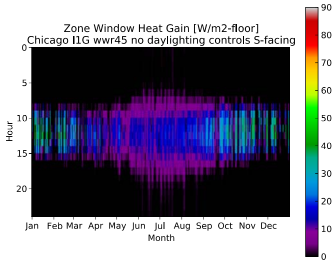
Figure 18. Hourly window heat gains with three different angular selective layers in identical IGUs, for south-facing perimeter zones in Chicago and WWR=0.45.
