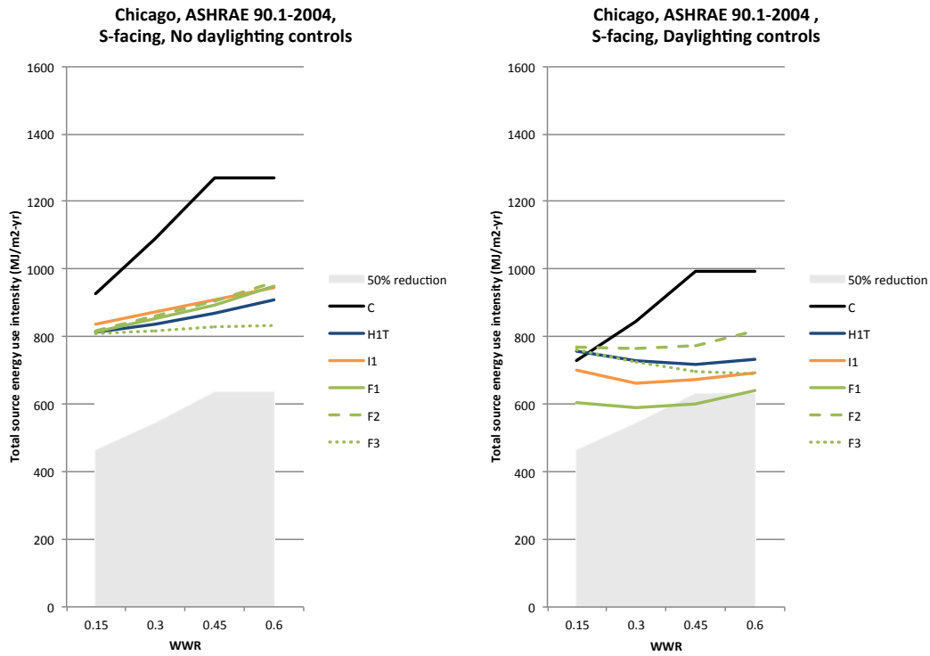
Figure 11. Annual source energy use intensity of triple-paned angular selective configurations and “best-practice” window for south-facing perimeter zones in Chicago, with and without daylighting controls.
