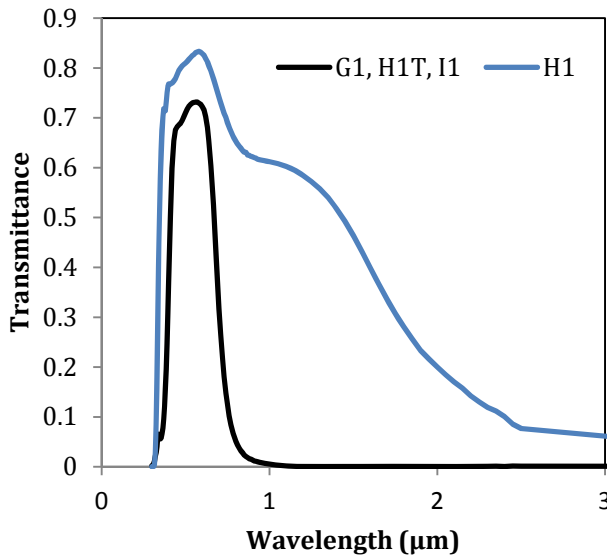
Figure 9. Spectral transmittance of coated glass in used in four angular-selective windows.
