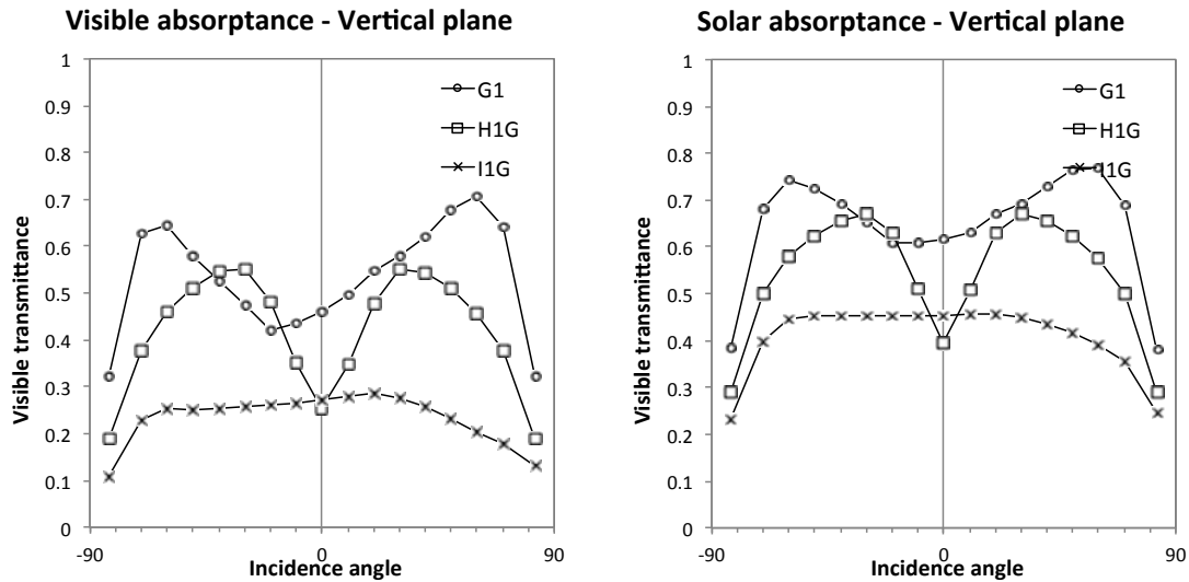
Figure 19. Directional-hemispherical visible and solar absorptance vs. angle of incidence across vertical plane for angular selective system layers with identical IGU.
