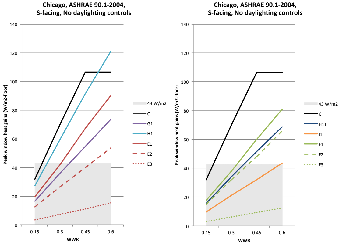
Figure 12. Peak window heat gains of angular selective systems and “best-practice” windows for south-facing perimeter zones in Chicago, without daylighting controls.
