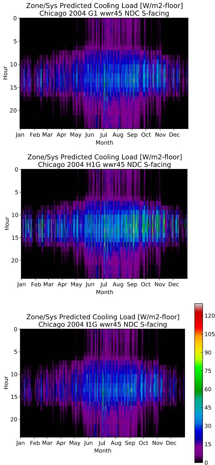
Figure 16. Hourly predicted cooling load with three different angular selective layers in identical IGUs, for south-facing perimeter zones in Chicago and WWR=0.45.
