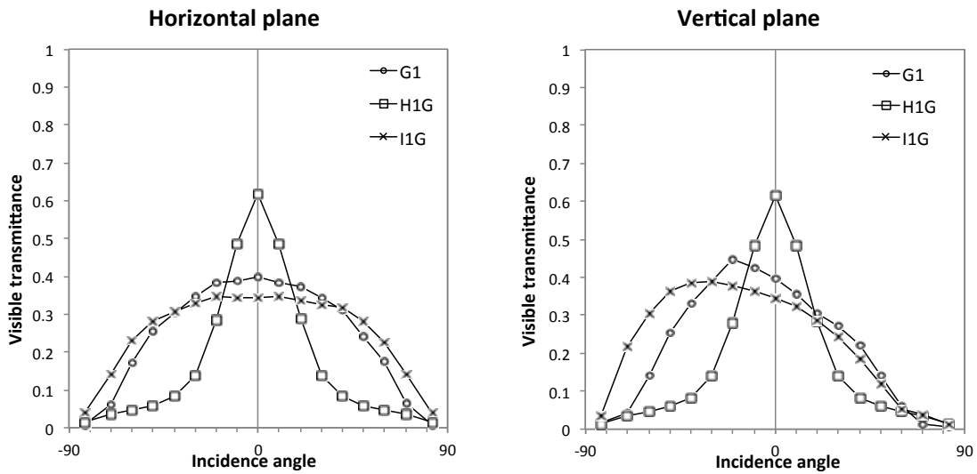
Figure 15. Directional-hemispherical visible transmittance vs. angle of incidence across vertical and horizontal planes for angular selective system layers with identical IGU.
