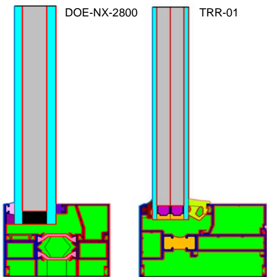
Figure 6. Cross-sectional diagrams of the two frame types.
