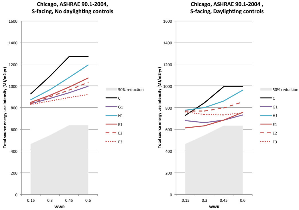
Figure 10. Annual source energy use intensity of double-paned angular selective system configurations and “best-practice” window for south-facing perimeter zones in Chicago, with and without daylighting controls.
