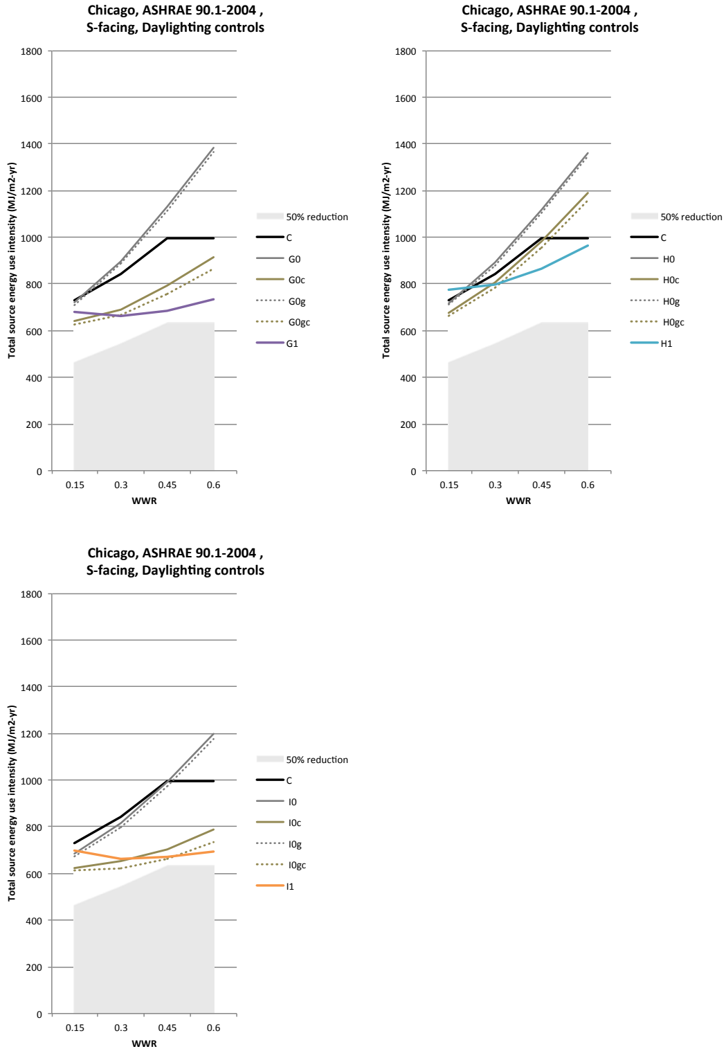
Figure 13. Annual source energy use intensity of angular selective system components for south-facing perimeter zones in Chicago, with daylighting controls.
