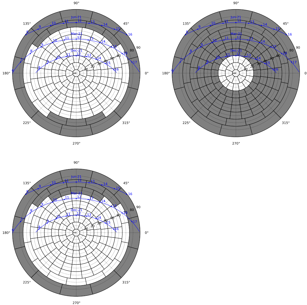
Figure 20. Shading diagrams for the three different angular selective layers in identical IGUs, facing south at latitude 42° N (Chicago): microperforated screen (G1) ( top left ), tubular shading structure (H1G) ( top right ), expanded metal mesh (I1G) ( bottom left ). Shaded sectors represent visible straight-through transmission of 2% or less.
