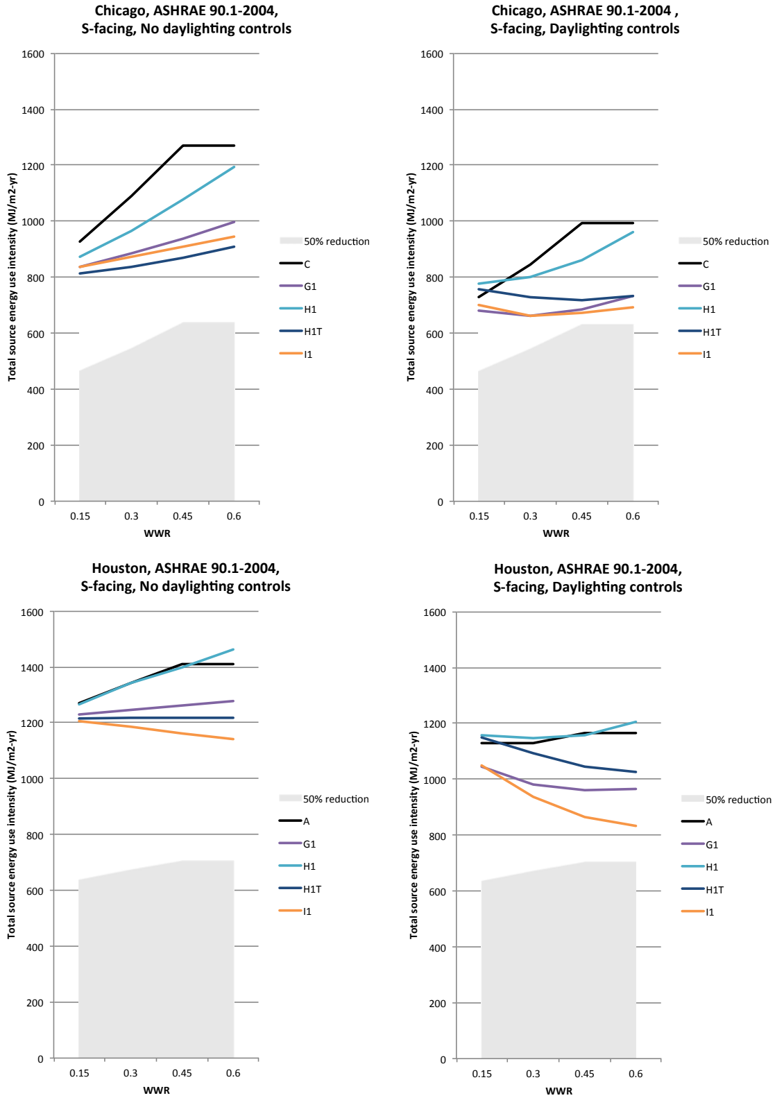
Figure 7. Annual source energy use intensity of angular selective systems and benchmark window for south-facing perimeter zones in Chicago and Houston, with and without daylighting controls.
