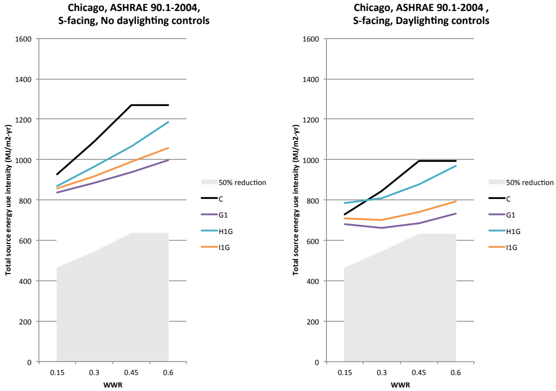
Figure 14. Annual source energy use intensity of angular selective system layers with identical IGU for south-facing perimeter zones in Chicago, with and without daylighting controls.
