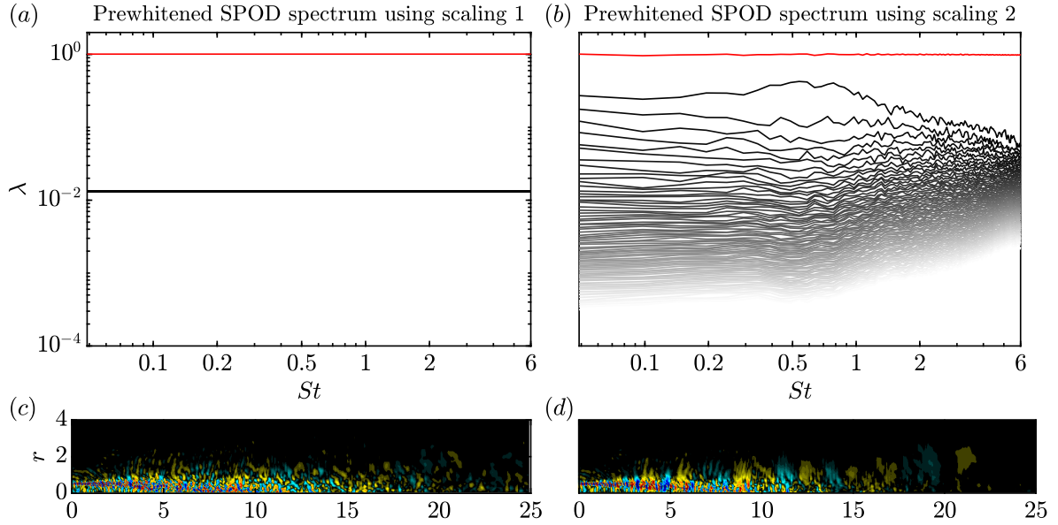
Figure 2.18: SPOD-based prewhitening: (a, b) rescaled SPOD spectra; (c, d) , instantaneous pressure fields using definitions (2.30) and (2.31), respectively. Red lines indicate the sum of all eigenvalues, that is, the integrated PSD. All lines in (a) collapse due to the scaling. The original SPOD eigenvalue spectrum can be seen in figure 2.2( a ).
