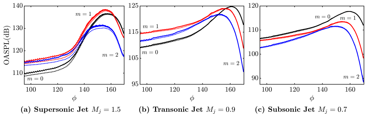
Figure 4.2.9: Comparison between OASPL of the LES pressure data (solid lines) and leading SPOD eigenvalue (dotted lines): m = 0 (black), m = 1 (red) and m = 2 (blue).
