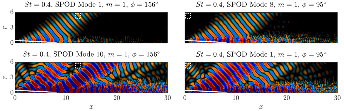
Figure 4.2.14: Comparison of leading and suboptimal SPOD modes for the supersonic jet M_j = 1.5 at St = 0.40 : mode 1 (top left) and mode 10 (bottom left) for \phi = 156^\circ ; mode 8 (top right) and mode 1 (bottom right) for \phi = 95^\circ . The most similar modes were identified by visual inspection.
