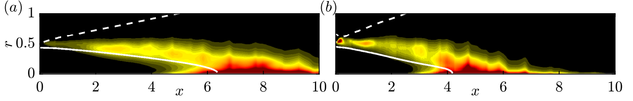
Figure 5.4.6: Integral interaction maps, \sum_{k,l} \lambda_1(St_k, St_l) |\phi_{k \circ l} \circ \phi_{k+l}| : (a) unforced turbulent jet; (b) forced turbulent jet. White solid and dashed lines outline the potential core and the jet width defined as lines of constant u_x = 0.95U_j and 0.05U_j , respectively.
