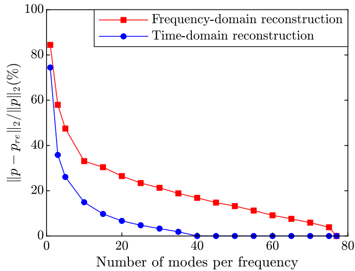
Figure 2.8: Two-norm error of the pressure field reconstructed with different rank approximation: (red lines with squares) reconstruction in the frequency domain; (blue lines with circles) reconstruction in the time domain.
