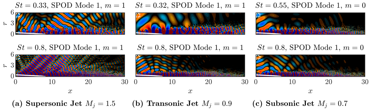
Figure 4.2.12: Leading SPOD modes at peak frequencies (top row) and for St = 0.80 (bottom row). The focus region is indicated by the dashed white box. White solid lines represent the edge of the potential core defined as \bar{u}(x, r) = 0.95U_j , where \bar{u} is the mean axial velocity.
