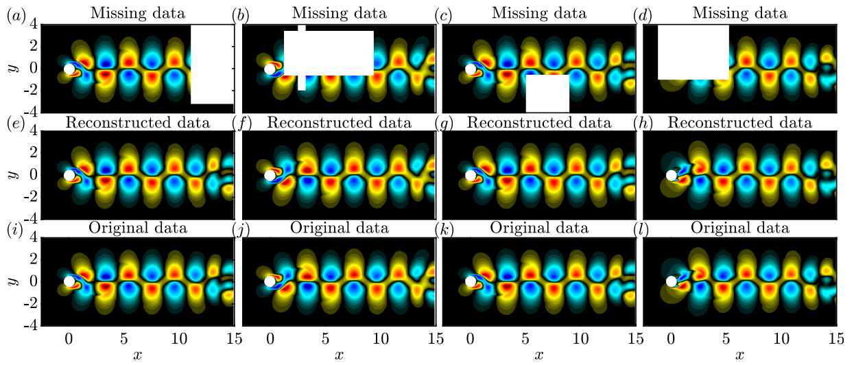
Figure 3.4.4: Reconstruction for 5% gappiness at four time instances: (a-d) gappy data; (e-h) reconstructed data; (i-l) original data. False colors of the streamwise velocity fluctuations, u , are on the same scale in all plots.
