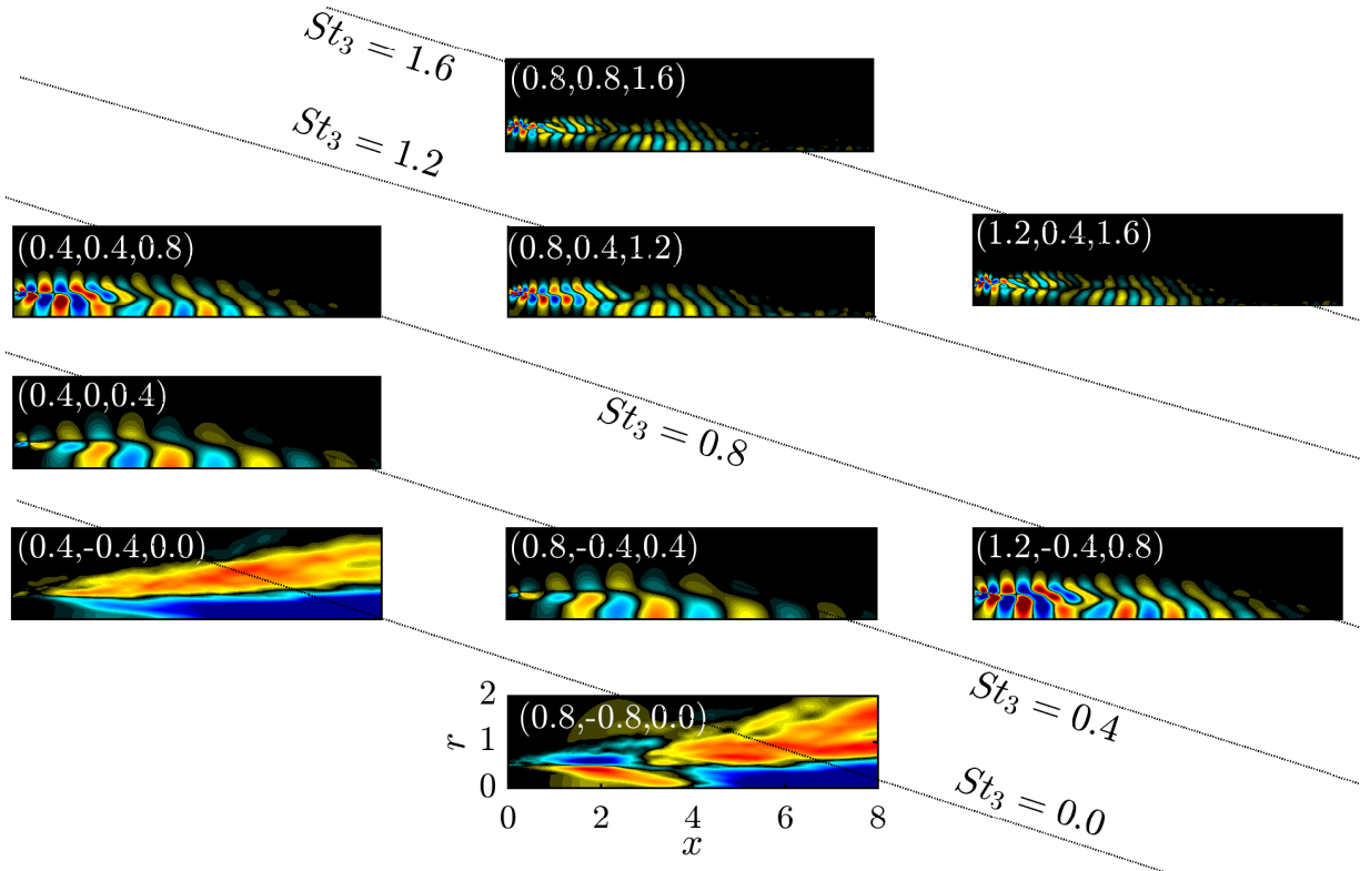
Figure 5.4.4: Bispectral modes forming a cascade of triads, starting from the forcing frequency (St_1, St_2, St_3) = (0.4, 0.0, 0.4) , middle-left. The real part of the streamwise velocity component is shown.
