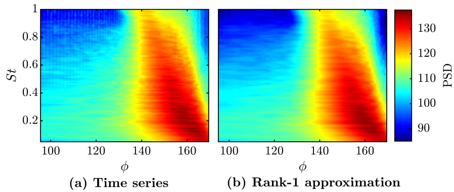
Figure 4.2.8: PSD estimated from the (a) time series of the LES pressure data and (b) leading SPOD eigenvalue for m = 0 of the supersonic jet.
