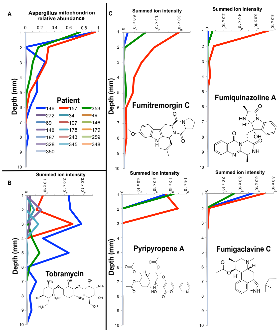
Fig. 5. Profiles of Aspergillus mitochondrion reads, tobramycin abundance, and Aspergillus specialized metabolite abundance through the WinCF oxygen gradients in the 19 patients tested in this study. (A) Relative abundance of 16S rDNA gene reads in each patient mapping to the Aspergillus mitochondrion in tobramycin-treated WinCF tubes through the 10-mm depth. (B) Summed ion intensity of tobramycin in each patient through the WinCF 10-mm depth treated with tobramycin. (C) Spectral counts of A. fumigatus specialized metabolites in same samples.
