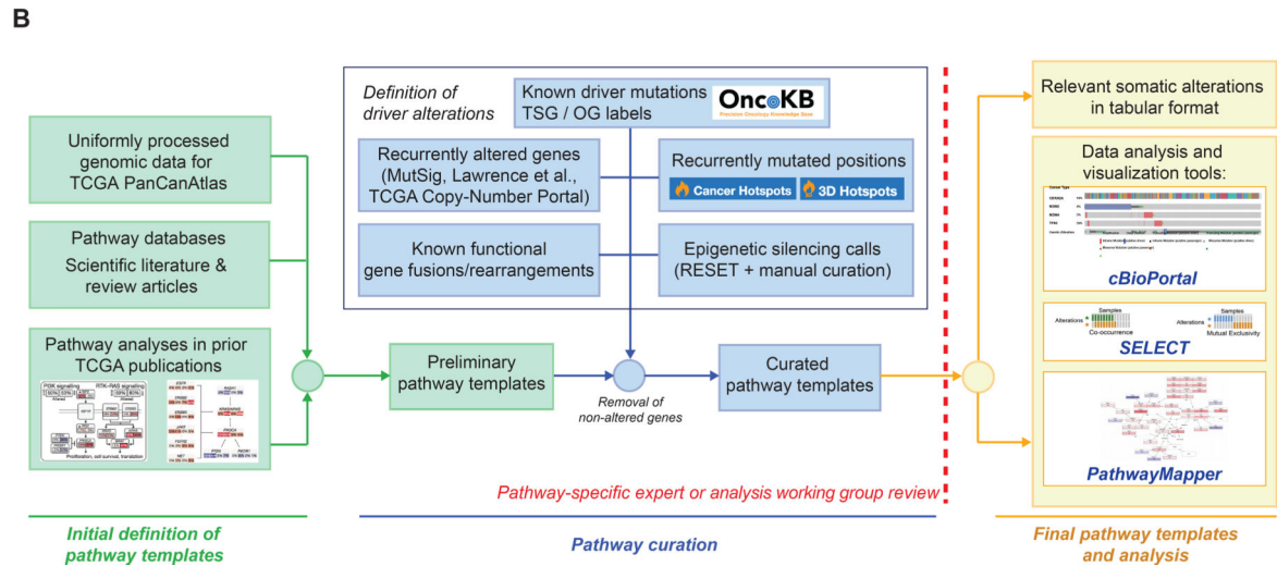
Figure 1. TCGA PanCanAtlas Pathways data set and workflow (A) Distribution of cancer types in the cohort, including molecular subtypes analyzed. (B) Workflow for pathway curation and analysis. Genes were curated from previous TCGA efforts and the scientific literature. Only genes with evidence for statistically recurrent or known driver alterations in the uniformly processed TCGA PanCanAtlas data set were included in the curated pathway templates. TCGA disease codes and abbreviations: AML: Acute Myeloid Leukemia; ACC:Adrenocortical carcinoma; BRCA:Breast cancer; CESC:Cervical cancer; KICH:Chromophobe renal cell carcinoma; KIRC:Clear cell kidney carcinoma; CRC: colorectal adenocarcinoma; SKCM:Cutaneous melanoma; DLBC:Diffuse
