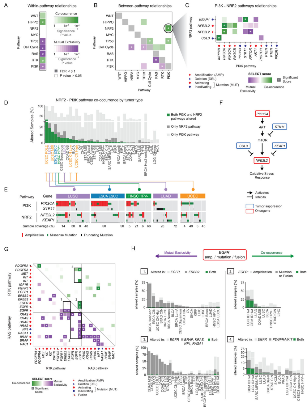
Figure 6. Co-occurrence and mutual exclusivity of pathway alterations A–B) Mutual exclusivity (purple) and co-occurrence (green) of gene alterations within pathways (A) and between pathways (B). Asterisks indicate significant relationships (Q value < 0.1). (C) Co-occurrence and mutual exclusivity of individual gene alterations in the PI3K and NRF2 pathways. (D) Breakdown of the co-occurrence of gene alterations in the PI3K and NRF2 pathways by tumor subtype. Green bars: percentage of samples with alterations in both PI3K and NRF2 pathways. Pathways are sorted by decreasing percentage of samples with alterations in both pathways. (E) Details of gene alterations in select genes ( PIK3CA , STK11 , NFE2L2 and KEAP1 ) within and between PI3K and NRF2 pathways,
