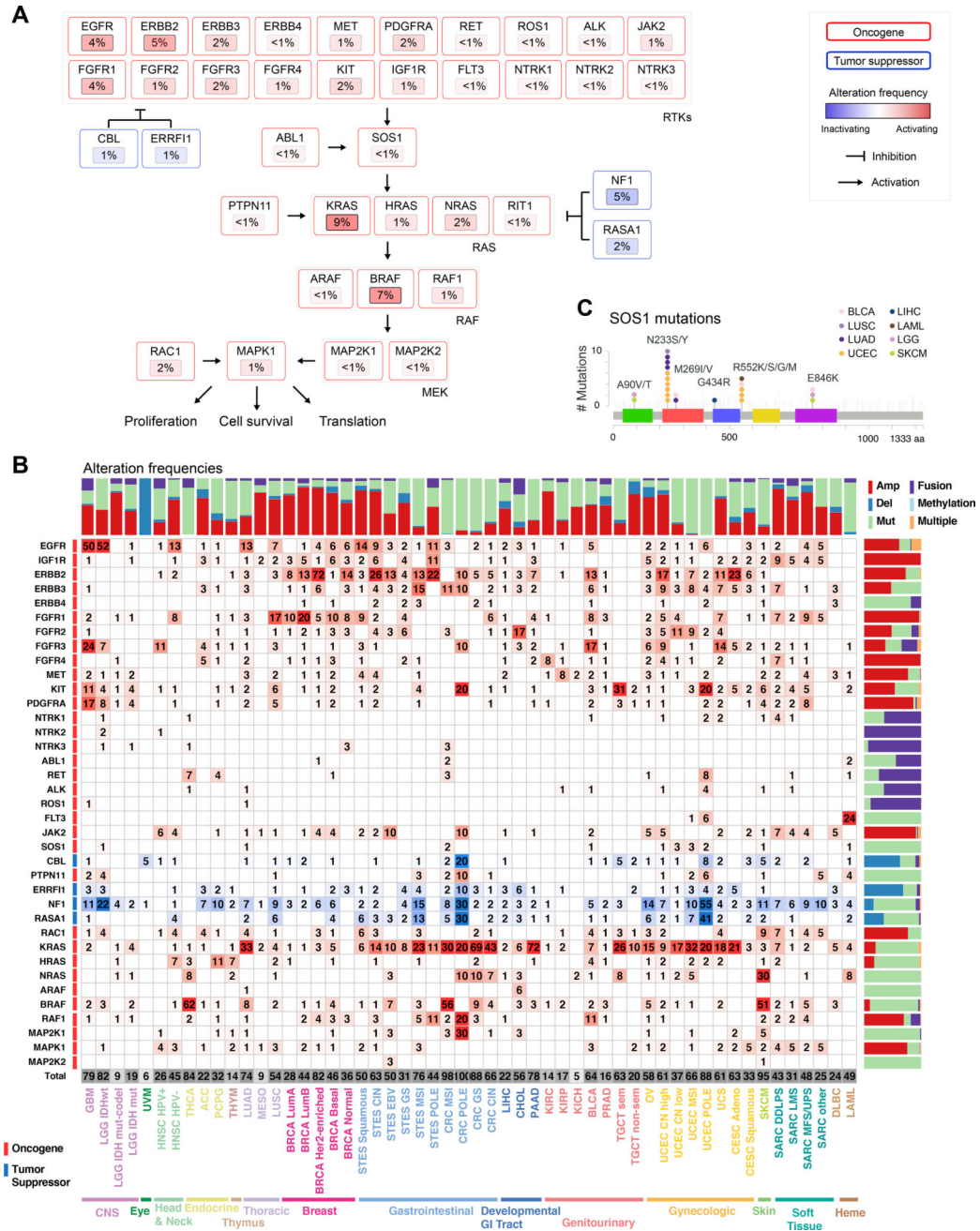
Figure 4. RTK-RAS pathway alterations (A) Altered genes and their functional relationships in the RTK-RAS pathway. Shades of red indicate frequencies of activating events (known or likely activating mutations or fusions, amplifications) and shades of blue indicate frequencies of inactivating events (known or likely inactivating mutations or fusions, homozygous losses). (B) Detailed heatmap of alteration frequencies in members of the RTK-RAS pathway. Only known or likely oncogenic alterations in each gene are considered, as described in Methods. The individual gene alteration frequencies may add up to more than the total for each tumor type, as some tumor samples may have multiple alterations. Color side bars show the fraction of samples
