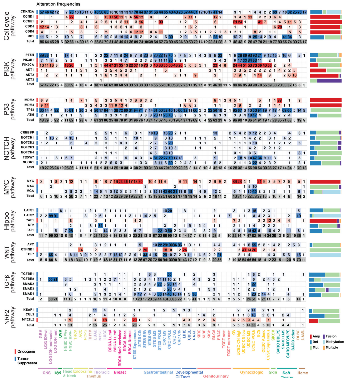
Figure 5. The most commonly altered genes in nine signaling pathways Oncogenic alteration frequencies per gene and tumor subtype for the most frequently altered genes in each pathway (for RTK-RAS see Figure 4). Red: activating events; blue: inactivating events; frequency of occurrence scale with color intensity. Last row for each pathway: overall alteration frequency of that pathway per tumor type. The individual gene alteration frequencies may add up to more than the total for each tumor type, as some tumor samples have multiple alterations. Color side bars show the fraction of samples affected by each type of somatic alteration (or a combination of them) for each pathway gene.
