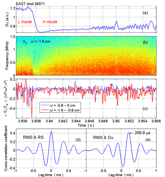
FIG. 3. (a) D\alpha emission near the inner target of the lower divertor, (b) time-frequency spectrum of a floating potential signal \Phi_{f1} at \sim 1.6 cm inside the separatrix, (c) turbulent Reynolds stress measured by a probe array near the separatrix ( \Delta r = -0.8 –0 cm, blue dashed curve) and another probe array deeper inside the plasma ( \Delta r = -1.6 – -0.8 cm, solid red curve). Cross-correlation coefficient between fluctuation RMS level of \Phi_{f1} and (d) radial gradient of the Reynolds stress, (e) D\alpha emission.
