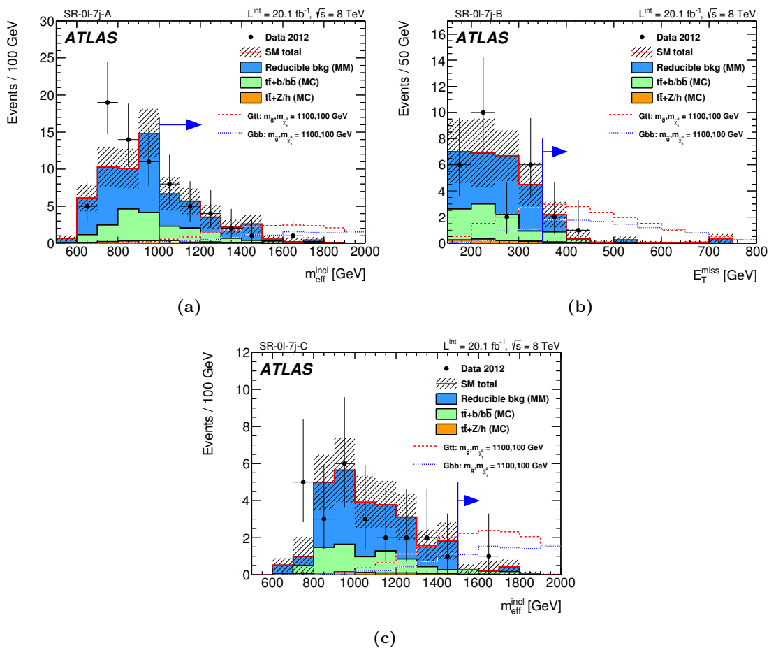
Figure 9. The (a)-(c) m_{\text{eff}}^{\text{incl}} and (b) E_T^{\text{miss}} distributions observed in data for SR-0 l -7j-A, SR-0 l -7j-B and SR-0 l -7j-C, respectively, after all requirements applied but the one indicated by the arrow, together with the background prediction. The shaded bands include all experimental systematic uncertainties on the background prediction. The prediction for two signal points from the Gtt ( \tilde{g} \rightarrow t\bar{t}\tilde{\chi}_1^0 ) and Gbb ( \tilde{g} \rightarrow b\bar{b}\tilde{\chi}_1^0 ) models are overlaid. The normalisation of the irreducible background t\bar{t} + b/\bar{b}b is as predicted by its theoretical cross-section scaled to the same luminosity as the data, prior to the fit in the control region.
