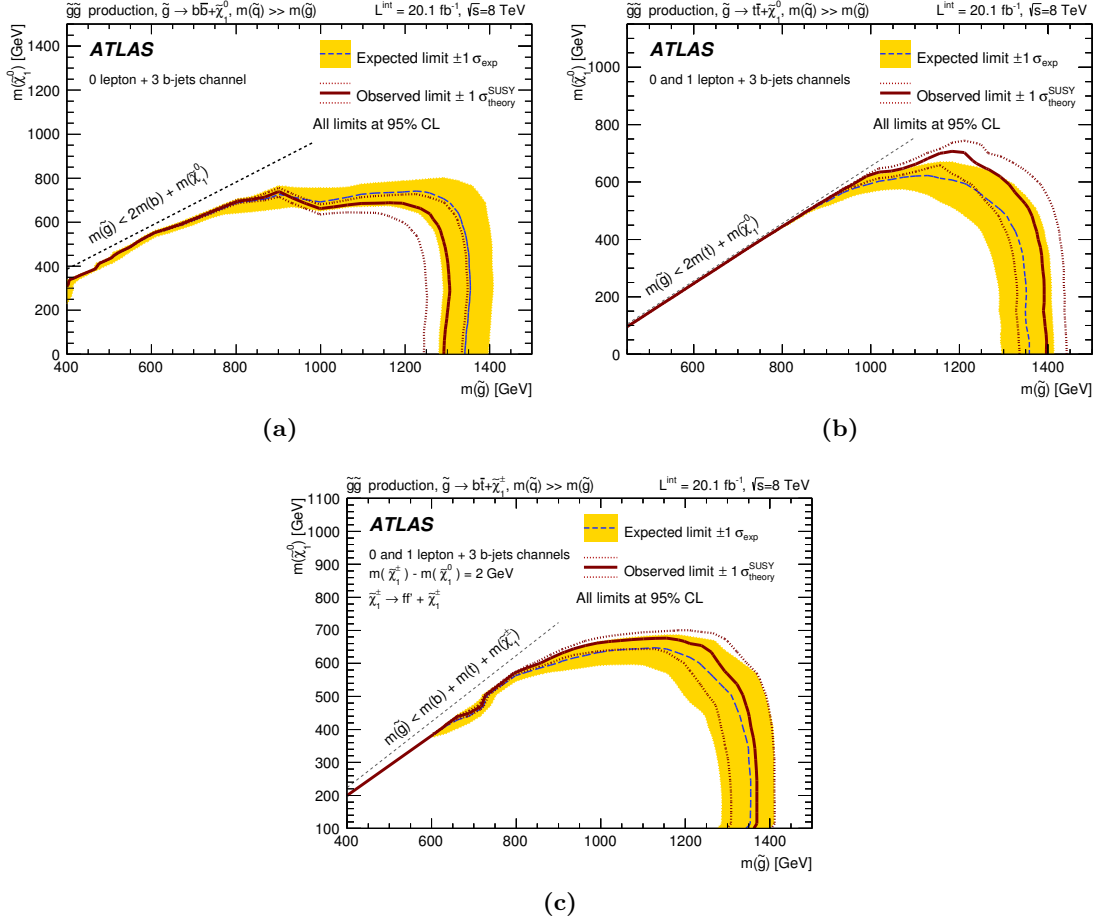
Figure 13. Exclusion limits in the (m_{\tilde{g}}, m_{\tilde{\chi}_1^0}) plane for the (a) Gbb, (b) Gtt and (c) Gtb models. The dashed blue and solid bold red lines show the 95% CL expected and observed limits respectively, including all uncertainties except the theoretical signal cross-section uncertainty. The shaded (yellow) bands around the expected limits show the impact of the experimental and background theoretical uncertainties while the dotted red lines show the impact on the observed limit of the variation of the nominal signal cross-section by 1\sigma of its theoretical uncertainty.
