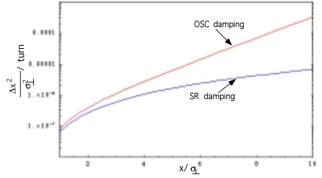
Figure 4: Critical diffusion versus the amplitude. Bottom curve shows only effect of synchrotron radiation (SR) damping. Top curve shows the combined effect of SR damping and OSC.
