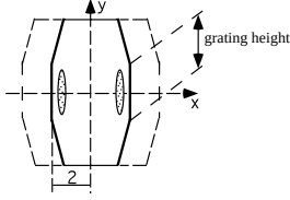
Figure 3: The cross-section of the vacuum chamber. Dashed lines show grating position at injection.
