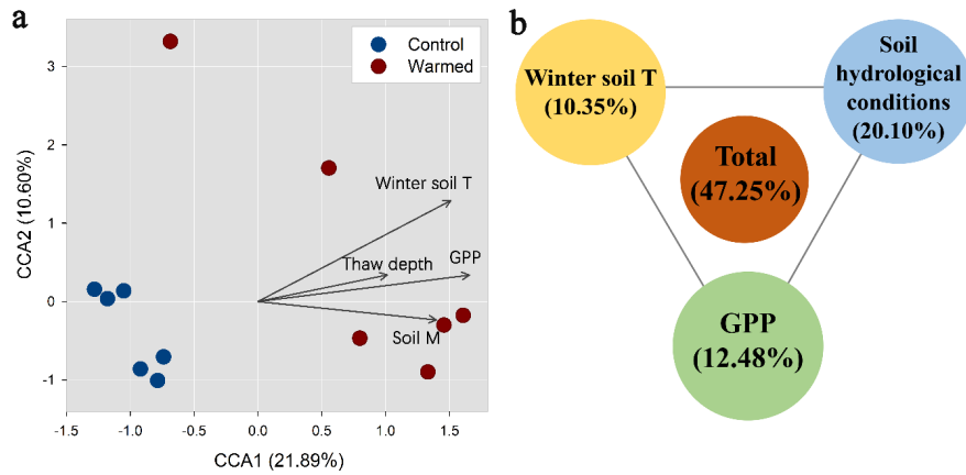
Figure 3. (a) Winter soil temperature (winter soil T), thaw depth, soil moisture (soil M) and gross primary productivity (GPP) are linked to fungal functional gene composition, as revealed by the canonical correlation analysis (CCA); (b) The variation partitioning analysis (VPA) shows explanatory percentages of environmental factors to fungal functional gene composition.
