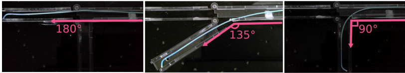
(b) VINE catheter
