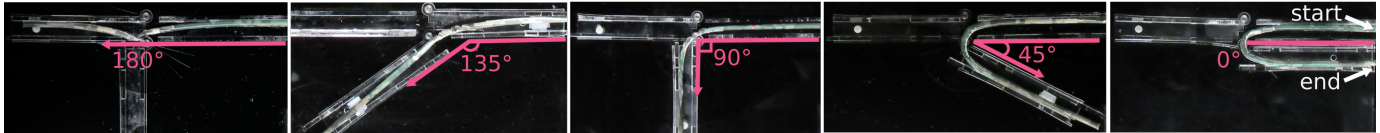
Fig. 5. (a) The standard semi-rigid catheter is only able to traverse curves as sharp as 90^\circ . (b) Device robustness to varying anatomies demonstrated by growing the VINE catheter through channels with angles ranging from 180^\circ (straight line on the left) to 0^\circ (complete u-turn on the right).
