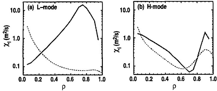
FIG. 6. Ion thermal diffusivity versus \rho , square root of the normalized toroidal flux. The solid lines are the experiment and the dashed lines are the calculated neoclassical values. Representative time during (a) the high power L-mode phase and (b) the H-mode phase in discharge 87977.
