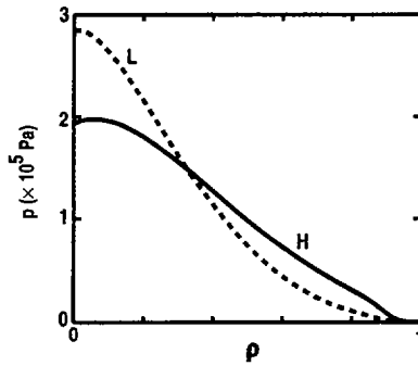
FIG. 3. Pressure profiles for discharges 87887 (L) and 87937 (H) at 2245 ms, showing the broadening of the H-mode versus \rho , the square root of toroidal normalized flux. The time evolution of these discharges is shown in Fig. 2.
