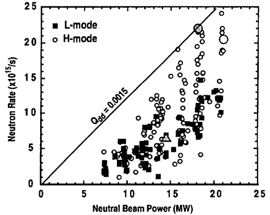
FIG. 4. Results from this experiment displayed as peak neutron rate, S_n , versus neutral beam power. The solid squares are L-mode plasmas and the open circles are H-mode. The large shaded circle is discharge 87977, discussed in Figs 5 and 6 and Table I. The large open circle is discharge 87937, shown in Figs 2 and 3.
