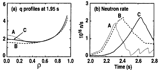
FIG. 5. Comparison of (a) "target" q -profiles before high-power heating and (b) time evolution of the neutron rate, in discharges 87977 (solid lines), 87937 (dashed lines), and 87953 (dotted lines).
