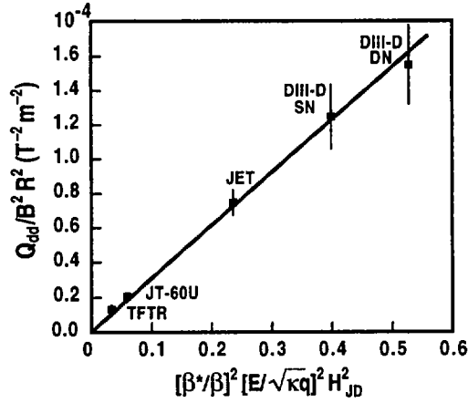
FIG. 7. Q_{dd}^* versus scaling relation discussed in the text for the highest DIII-D Q_{dd} and the highest values reported by TFTR, JET, and JT-60.
