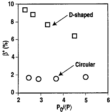
FIG. 1. Maximum \beta^* (fusion weighted \beta ) stable to the ideal n = 1 kink mode versus pressure peaking factor p_0/\langle p \rangle , for profiles of the form p = p_0(1 - \rho^2)^\alpha . Results are shown for a circular cross section and a D-shaped cross section with elongation 1.7 and triangularity 0.7.
