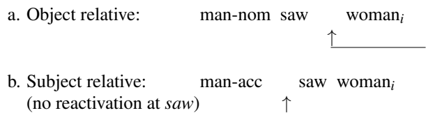
Figure 3: Temporal decay in Japanese (horizontal lines mark the material that contributes to decay; vertical arrows indicate the point in time the empty position is retrieved from)
