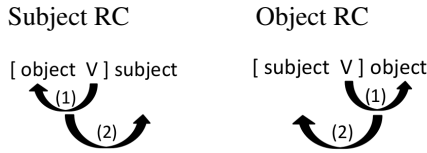
Figure 1: Order of semantic-role assignment in Japanese
