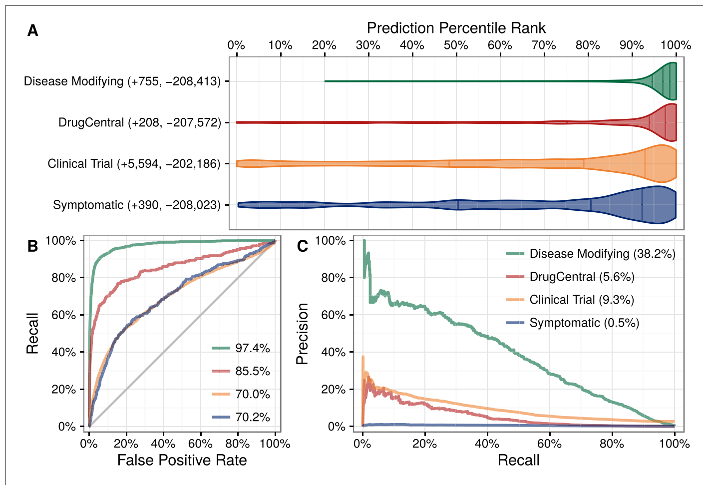
Figure 3. Predictions performance on four indication sets. We assess how well our predictions prioritize four sets of indications. (A) The y-axis labels denote the number of indications (+) and non-indications (–) composing each set. Violin plots with quartile lines show the distribution of indications when compound–disease pairs are ordered by their prediction. In all four cases, the actual indications were ranked highly by our predictions. (B) ROC Curves with AUROCs in the legend. (C) Precision–Recall Curves with AUPRCs in the legend.
